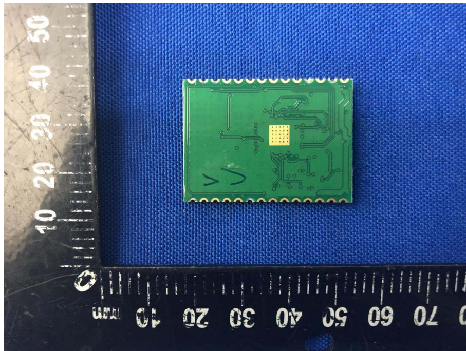
MAIN BOARD 3 REAR VIEW
