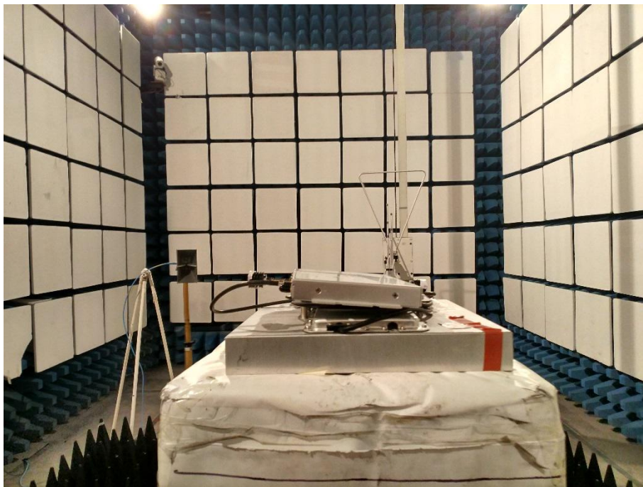
Close-up(RFID)
