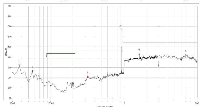
(Plot B.1: 30MHz to 10GHz, Antenna Horizontal @ Profile 0, channel 26)
