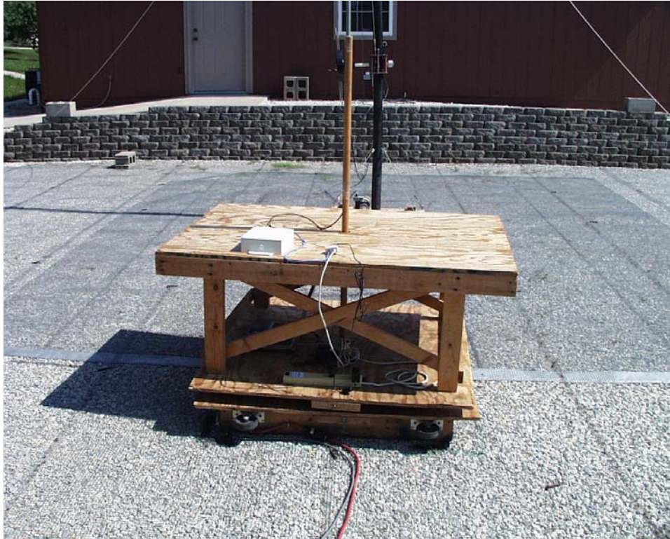
Test setup photographs for DLB23xx. Model DLB2310 photograph of radiated emissions test setup
