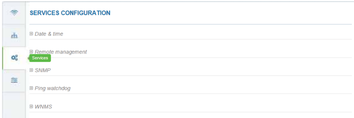
Figure 31 - Services Menu
