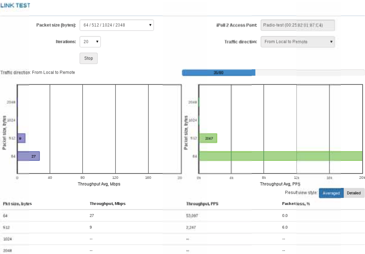
Figure 49 – Linktest Results
