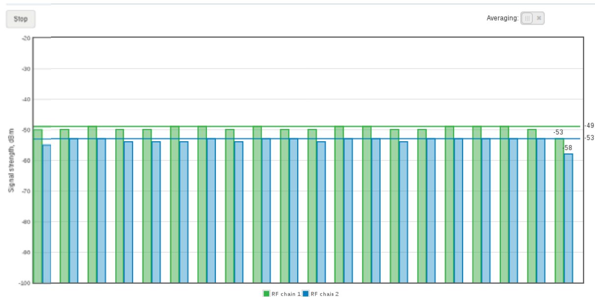
Figure 47 – Antenna Alignment
