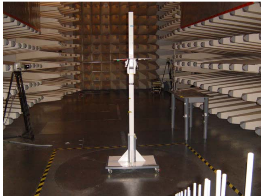
Set-up for Radiated Emission Test
