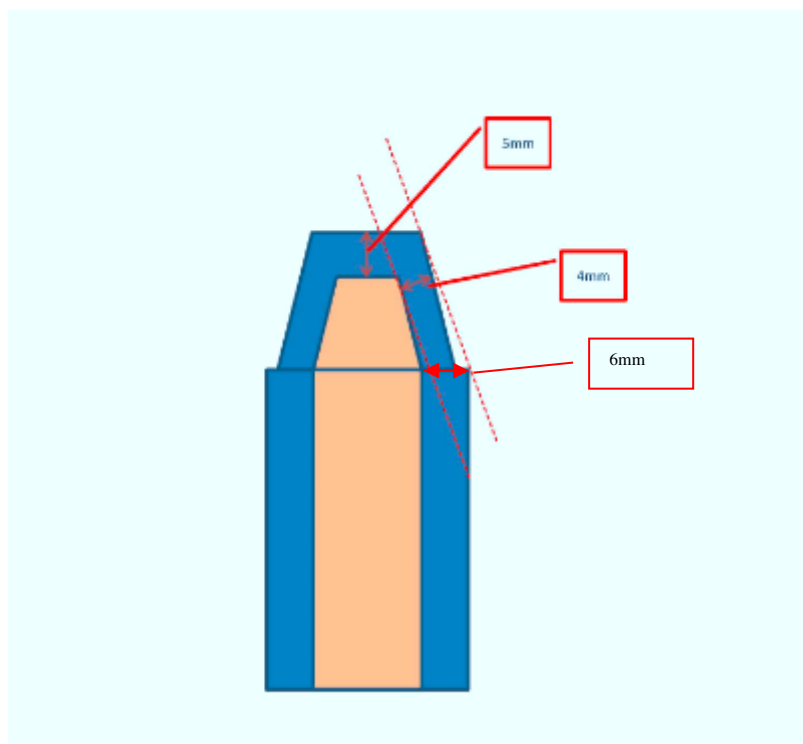
A(antenna location and the distances from antenna to head edge)
