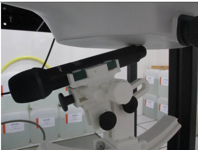
Body and Extremity SAR (Inclined)
