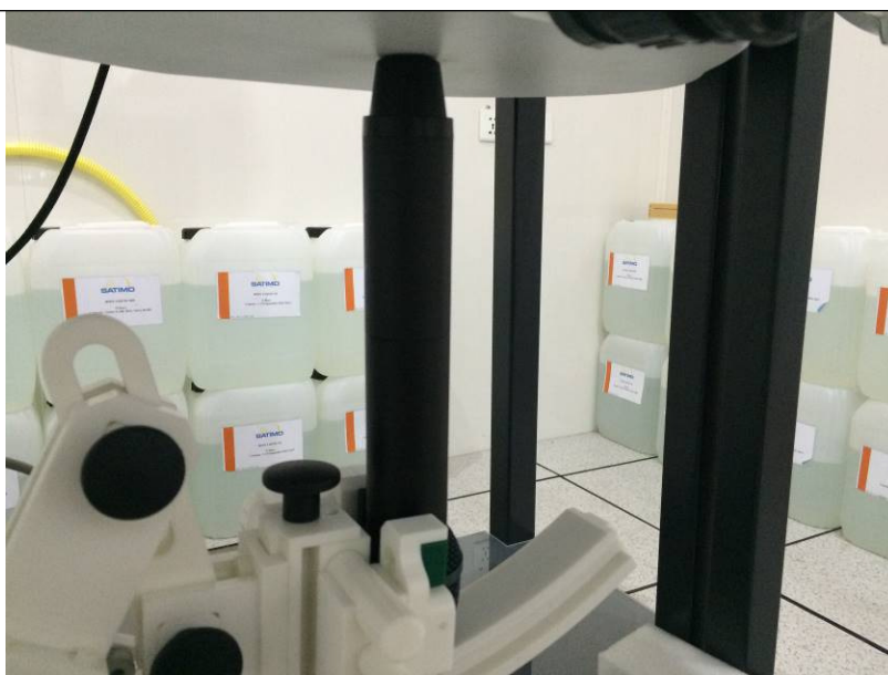
Body and Extremity SAR (Bottom)
