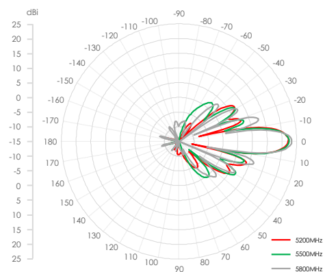
Elevation Plane
