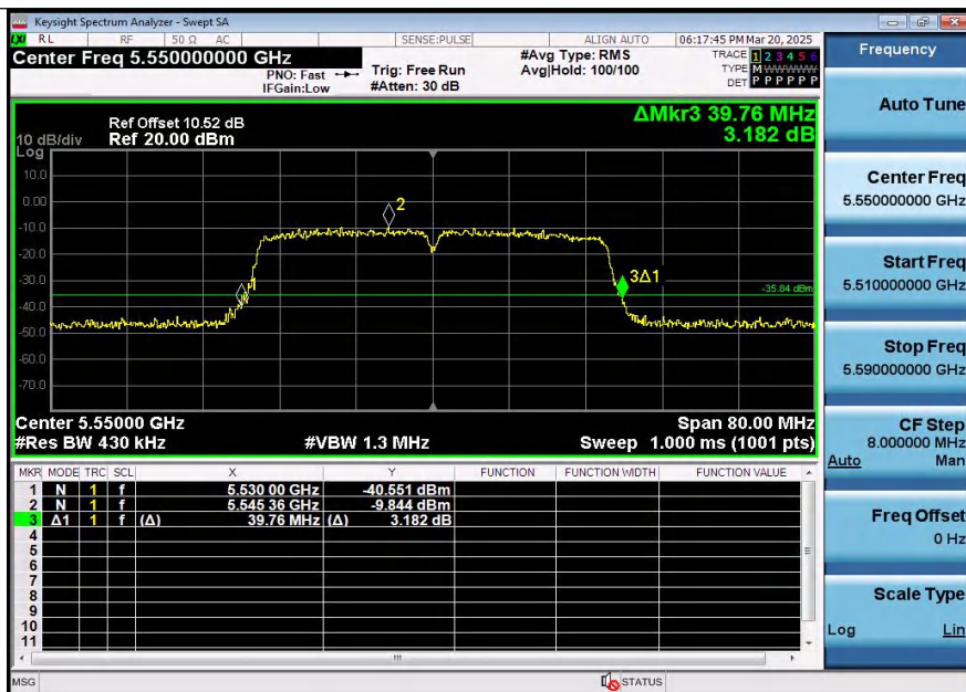
11AC40SISO-Ant2-5550
