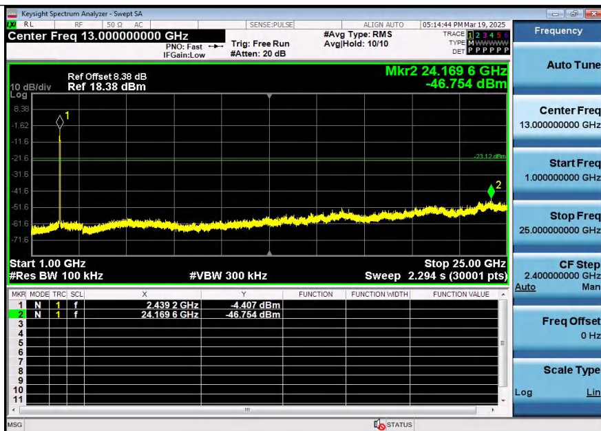
11AX40SISO-Ant2-2437-1000~25000-PASS
