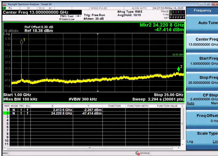
11AX20SISO-Ant2-2412-1000~25000-PASS
