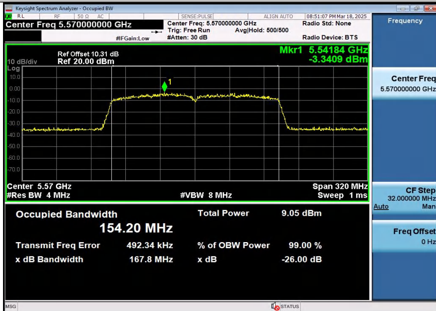
11AC160SISO-Ant2-5570
