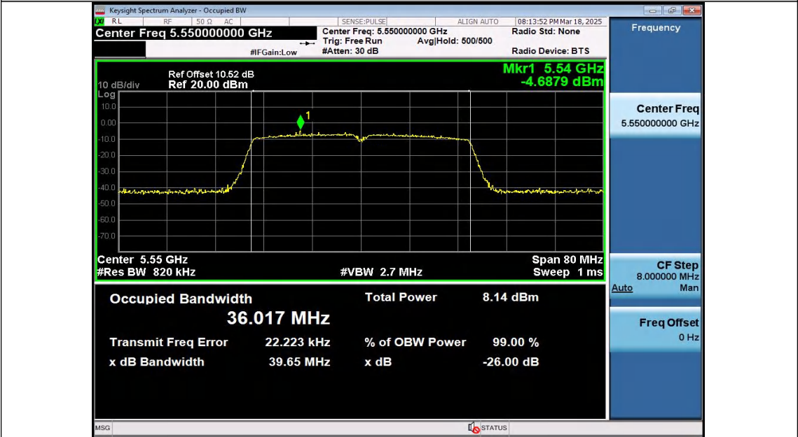
11N40SISO-Ant2-5550
