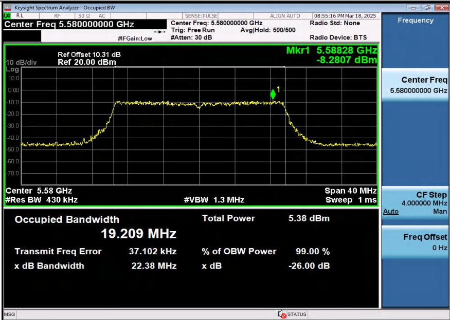
11AX20SISO-Ant2-5580
