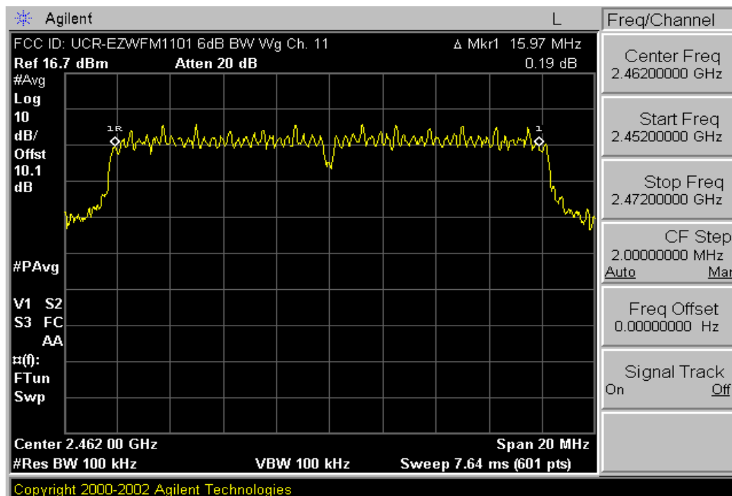
Plot 6-6. 6dB Bandwidth Plot (802.11g - Ch. 11)
