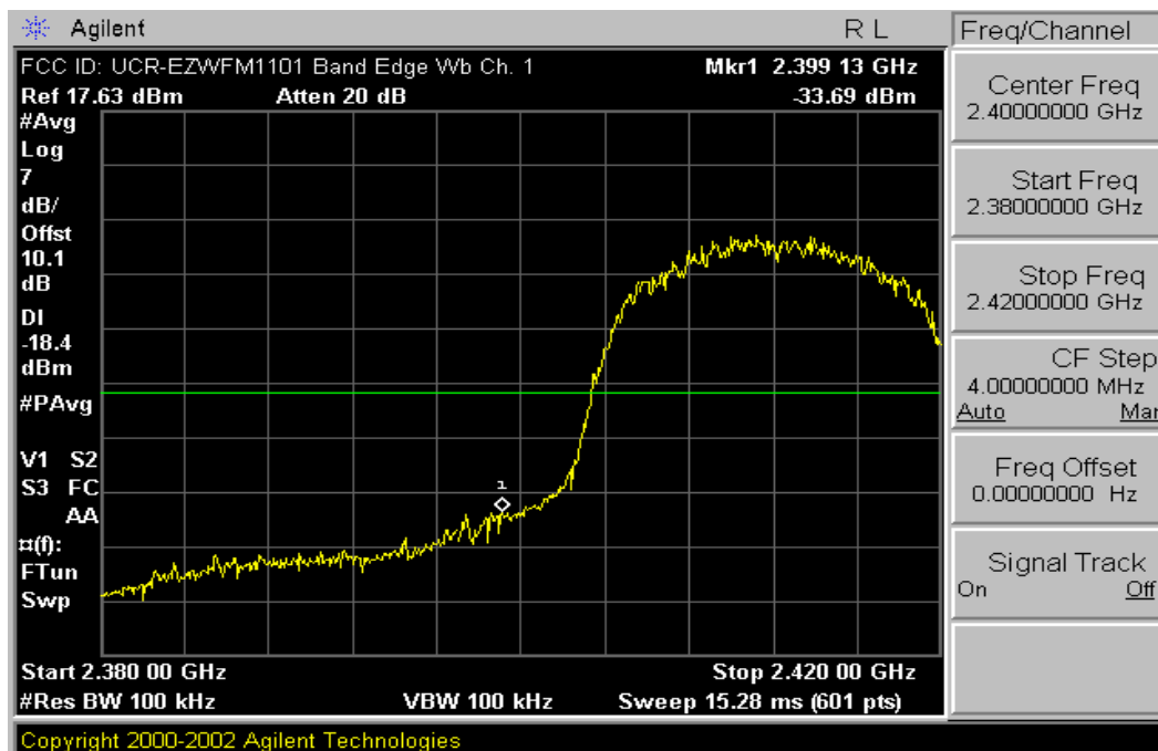
Plot 6-13. Band Edge Plot (802.11b – Ch. 1)
