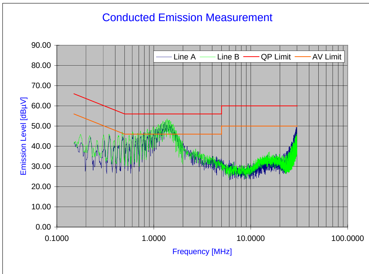
Plot 6-17. Line Conducted Plot with 802.11b
