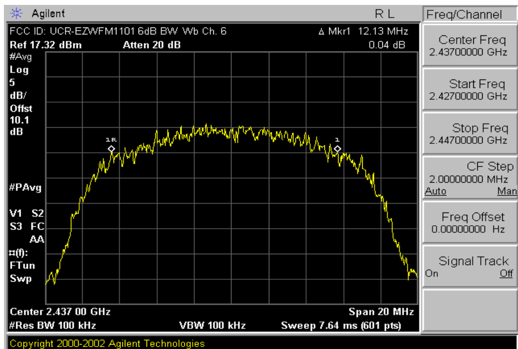
Plot 6-2. 6dB Bandwidth Plot (802.11b – Ch. 6)
