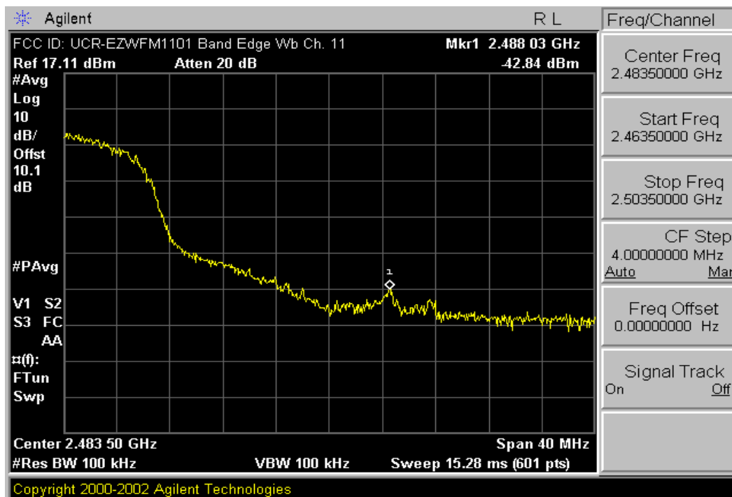
Plot 6-14. Band Edge Plot (802.11b – Ch. 11)
