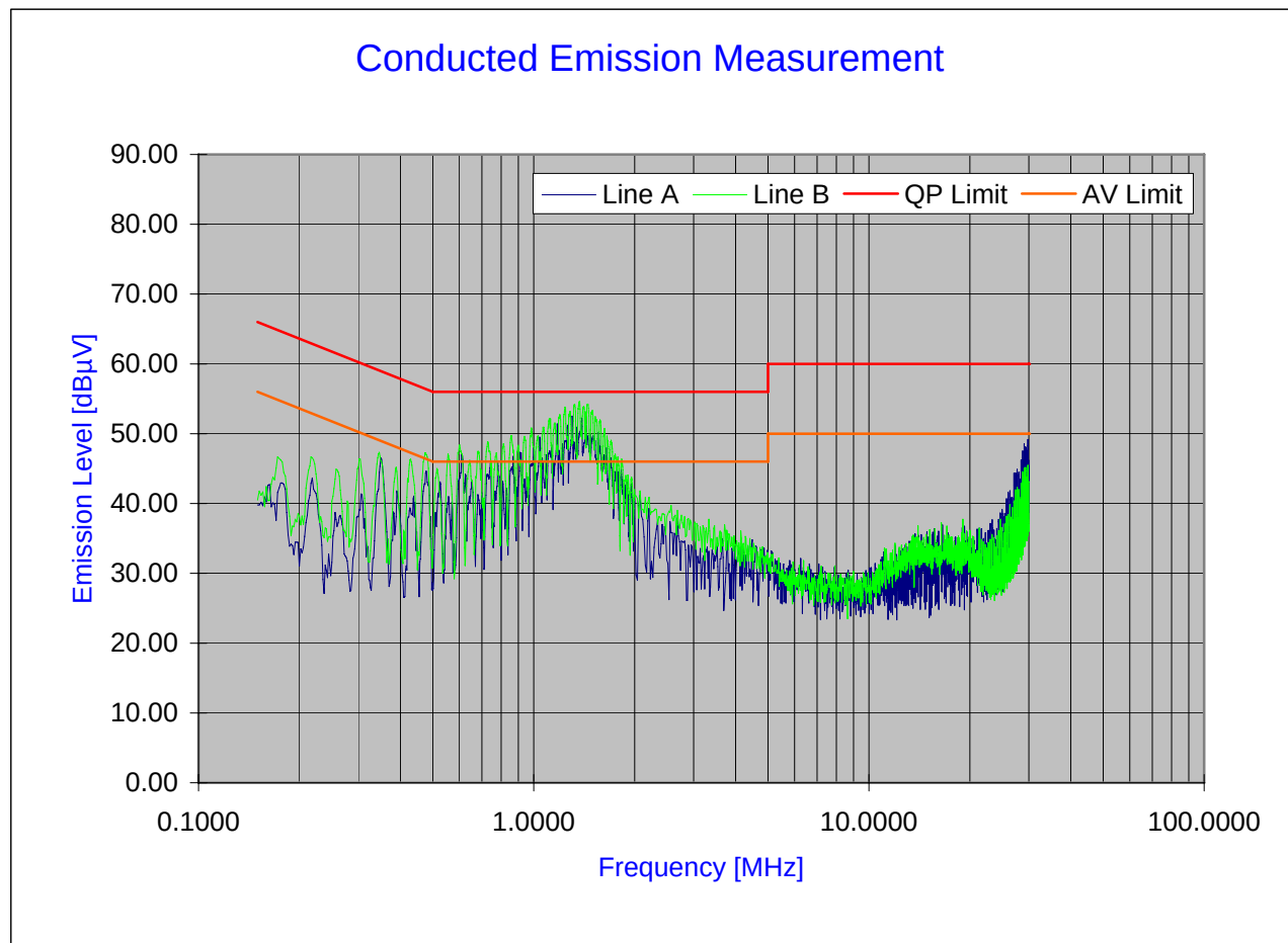
Plot 6-18. Line Conducted Plot with 802.11g
