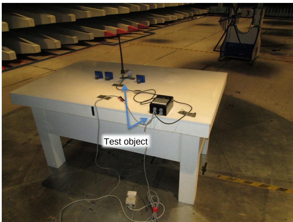
Photo 0.2 Test setup regarding measurement of peak output field strength of fundamental.
