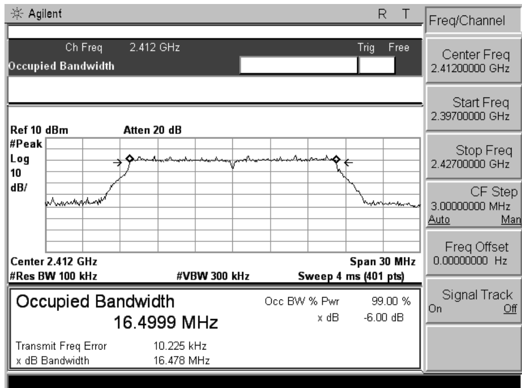
802.11g channel, 6dB bandwidth &amp; 99% Occupied Bandwidth
