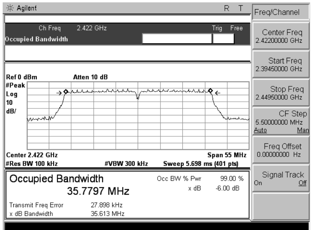
802.11n HT40 channel, 6dB bandwidth &amp; 99% Occupied Bandwidth
