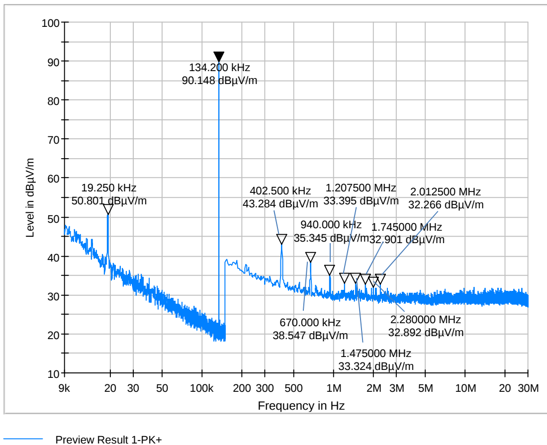
Figure 4.1.1 Preview measurement in semi anechoic chamber. Note; performed with peak detector.
