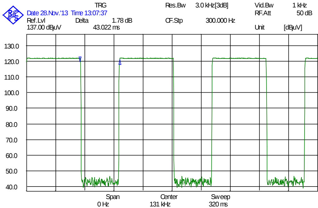
Duty cycle ON time with transponder
