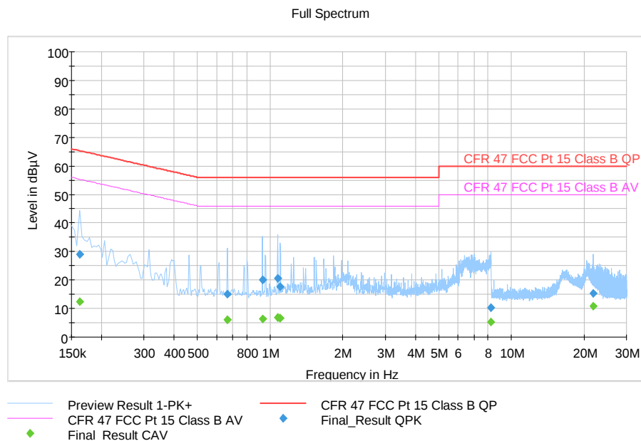
Power line conducted emissions spectrum
