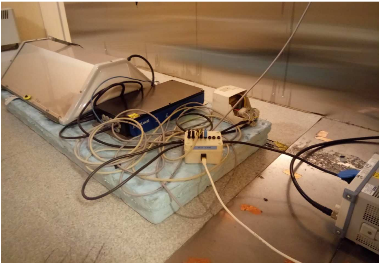
Conducted Emissions
