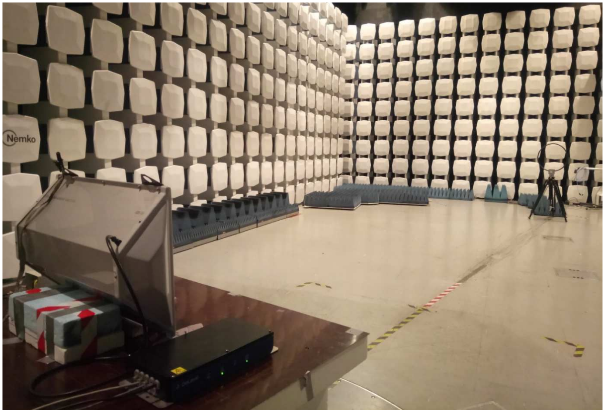
Radiated Emissions Below 30MHz, @10m
