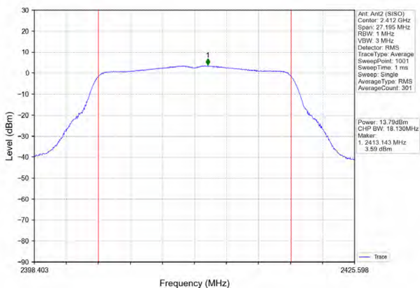
802.11g LCH 2412MHz Ant2 (SISO) NTNV
