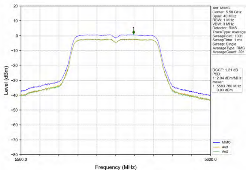
802.11n(HT20)_MCH_5580MHz_MIMO_NTN
