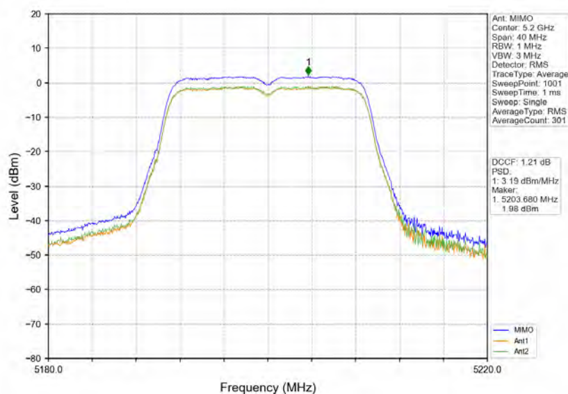
802.11n(HT20)_MCH_5200MHz_MIMO_NTN
