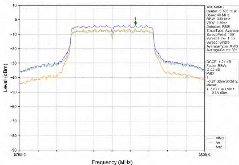
802.11n(HT20)_MCH_5785MHz_MIMO_NTN
