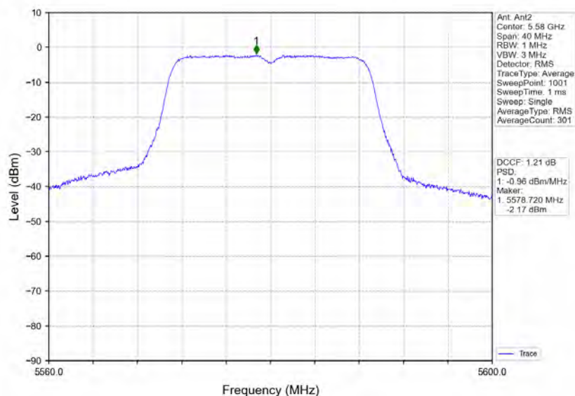
802.11n(HT20)_MCH_5580MHz_MIMO_NTN
