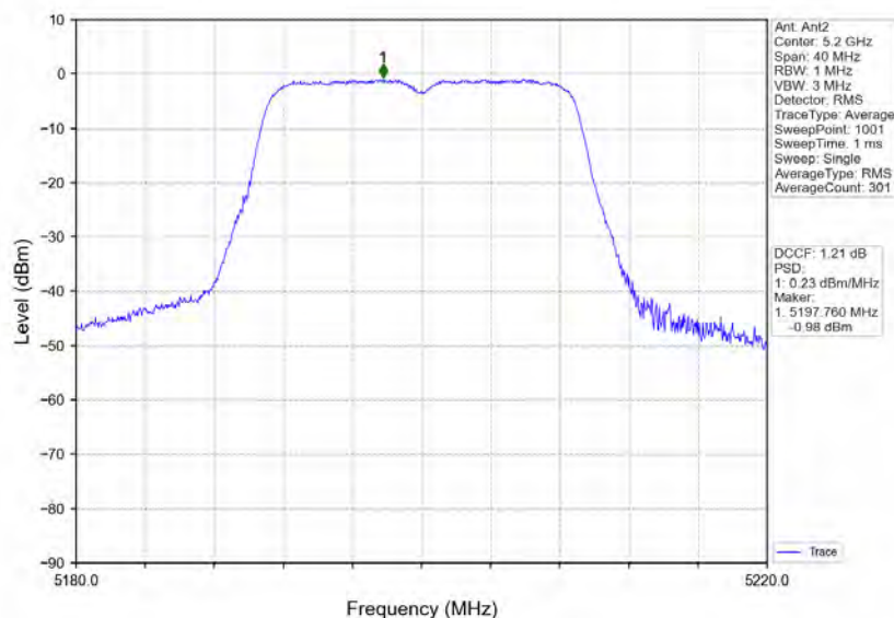
802.11n(HT20)_MCH_5200MHz_MIMO_NTN
