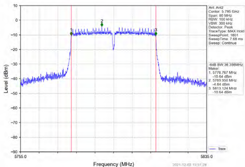
802.11ac(VHT40)_HCH_5795MHz_Ant2_NTNV
