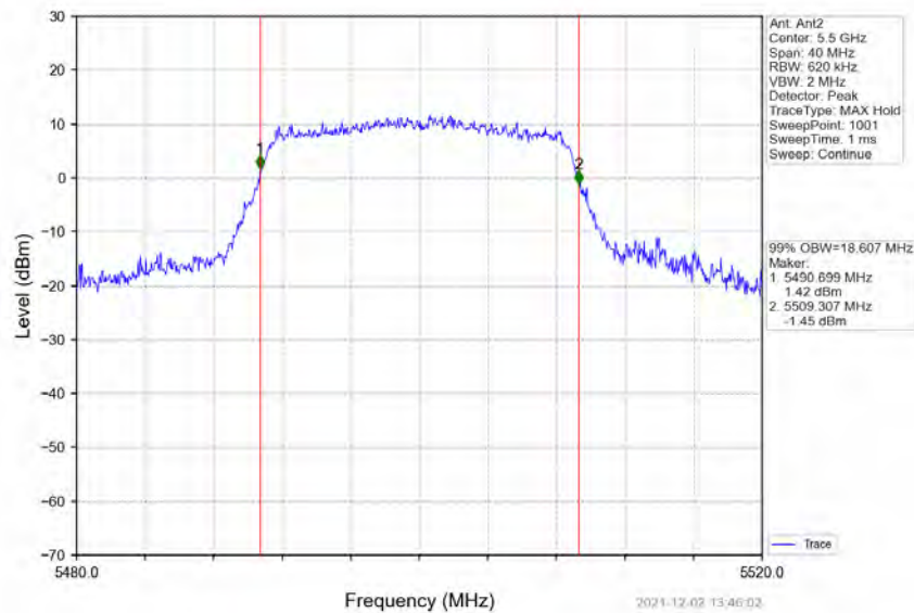
802.11ac(VHT20)_LCH_5500MHz_Ant2_NTNV
