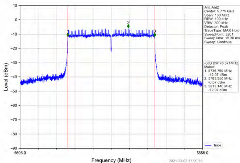
802.11ac(VHT80)_MCH_5775MHz_Ant2_NTNV
