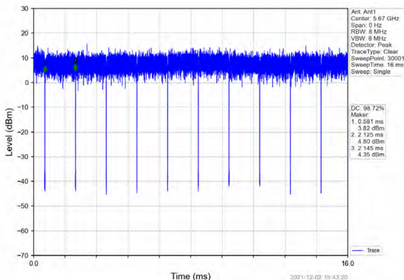
802.11ac(VHT40)_HCH_5670MHz_Ant1_NTNV
