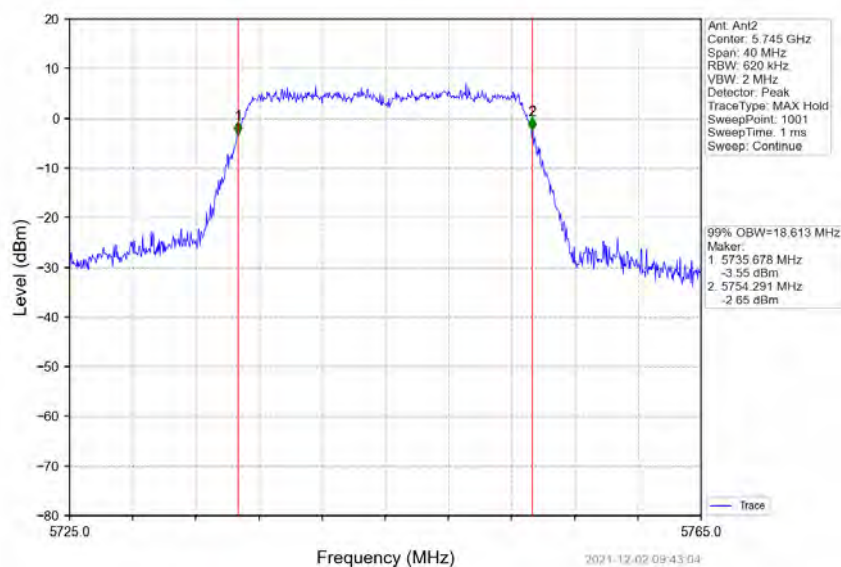
802.11n(HT20)_LCH_5745MHz_Ant2_NTNV
