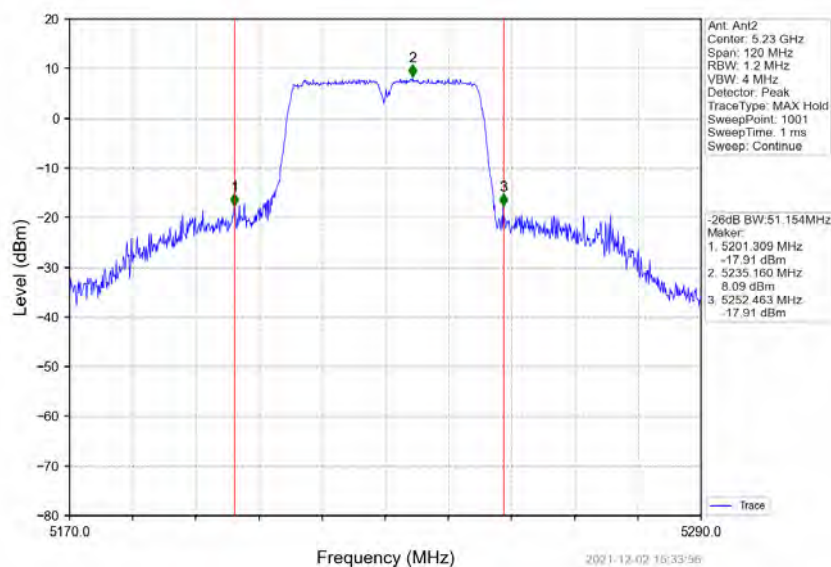
802.11ac(VHT40)_HCH_5230MHz_Ant2_NTNV
