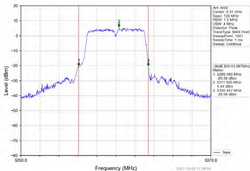
802.11n(HT40)_HCH_5310MHz_Ant2_NTNV
