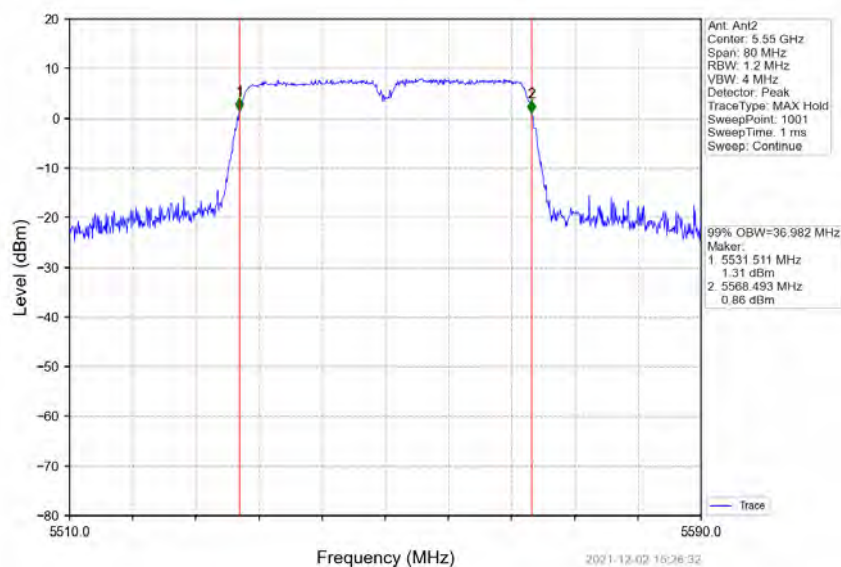
802.11ac(VHT40)_MCH_5550MHz_Ant2_NTNV
