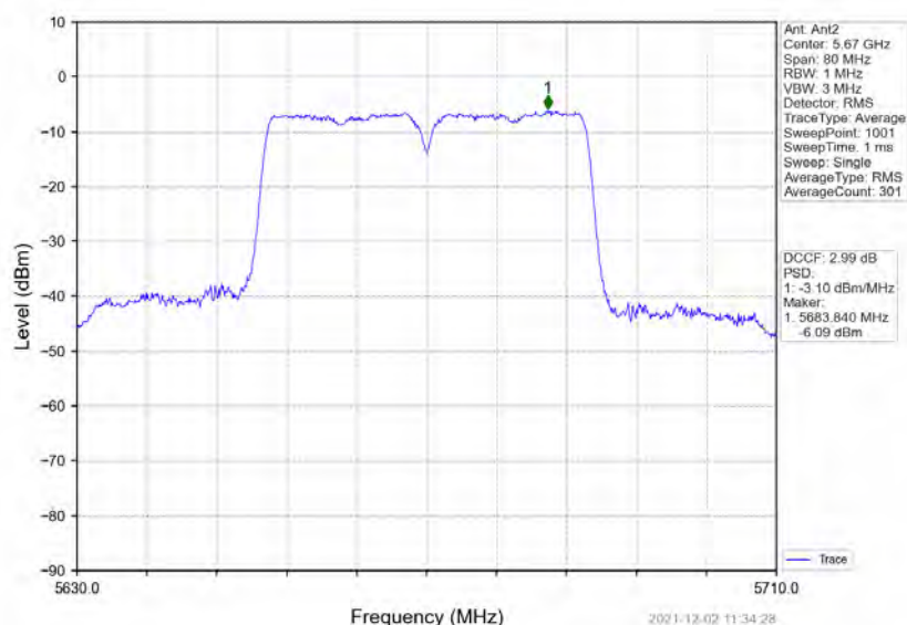
802.11n(HT40)_HCH_5670MHz_MIMO_NTNV
