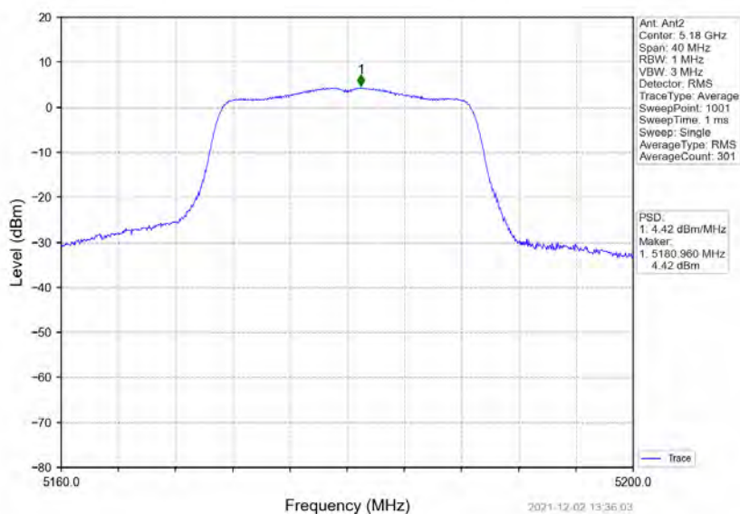
802.11ac(VHT20)_LCH_5180MHz_Ant2_NTNV
