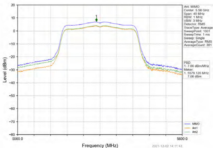
802.11ac(VHT20)_MCH_5580MHz_MIMO_NTNV
