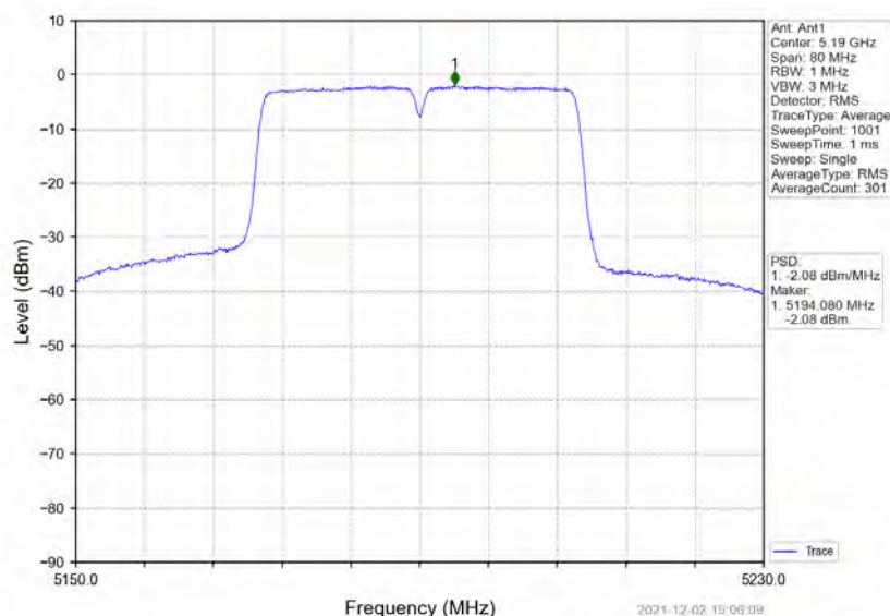
802.11ac(VHT40)_LCH_5190MHz_Ant1_NTNV
