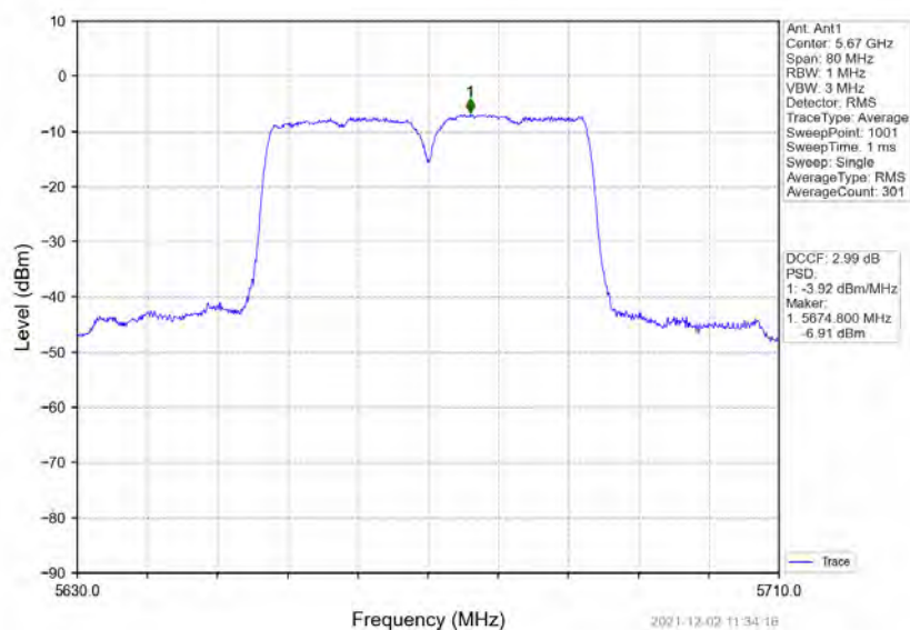
802.11n(HT40)_HCH_5670MHz_Ant1_NTNV
