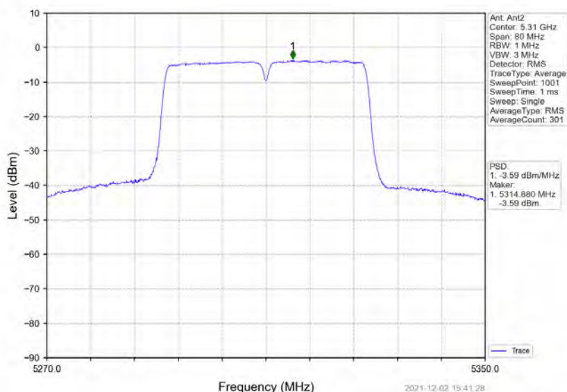
802.11ac(VHT40)_HCH_5310MHz_Ant2_NTNV
