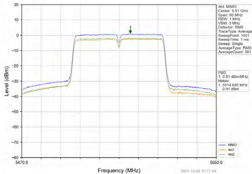
802.11ac(VHT40)_LCH_5510MHz_MIMO_NTNV
