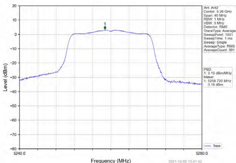
802.11ac(VHT20)_LCH_5260MHz_MIMO_NTNV
