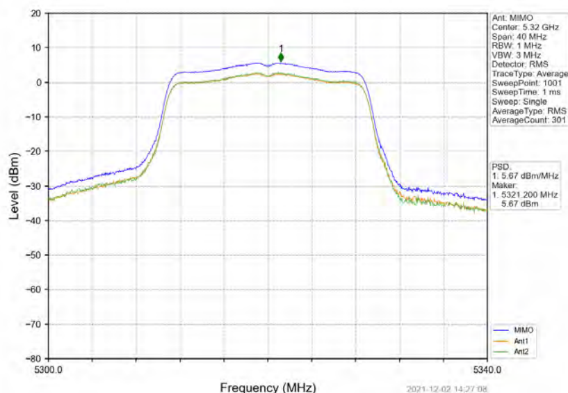
802.11ac(VHT20)_HCH_5320MHz_MIMO_NTNV
