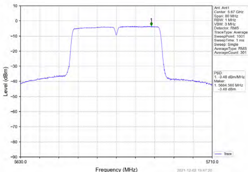
802.11ac(VHT40)_HCH_5670MHz_Ant1_NTNV
