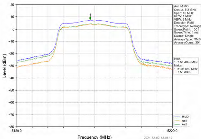
802.11ac(VHT20)_MCH_5200MHz_MIMO_NTNV
