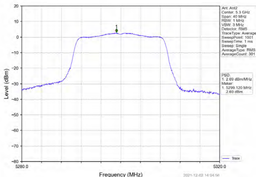
802.11ac(VHT20)_MCH_5300MHz_Ant2_NTNV
