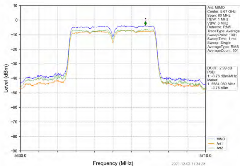
802.11n(HT40)_HCH_5670MHz_MIMO_NTNV
