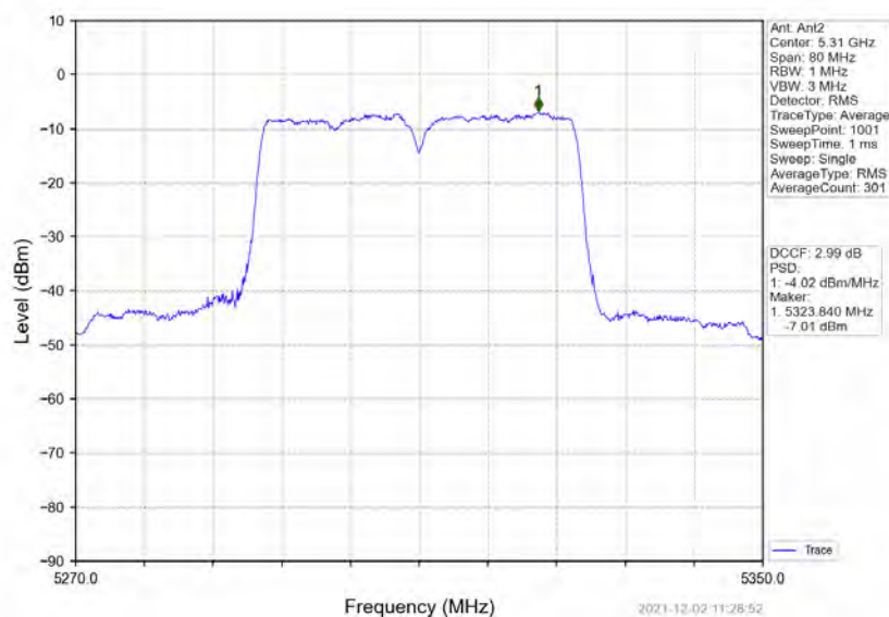
802.11n(HT40)_HCH_5310MHz_Ant2_NTNV
