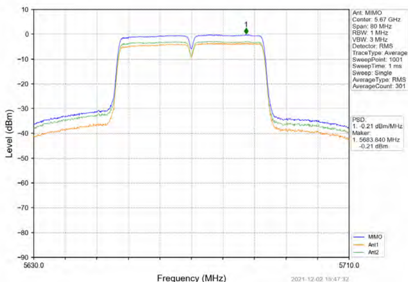
802.11ac(VHT40)_HCH_5670MHz_MIMO_NTNV
