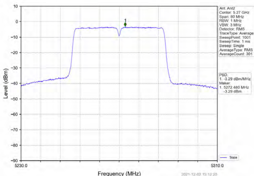
802.11ac(VHT40)_LCH_5270MHz_MIMO_NTNV
