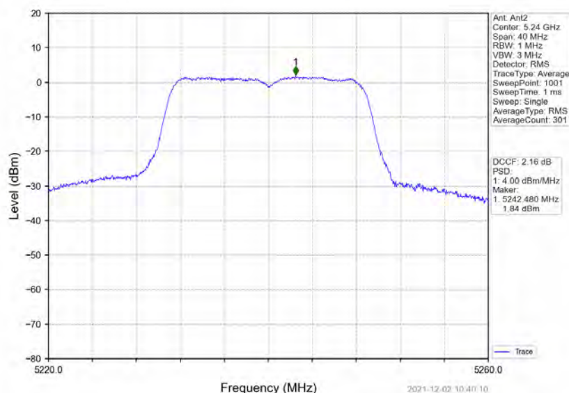
802.11n(HT20)_HCH_5240MHz_Ant2_NTNV
