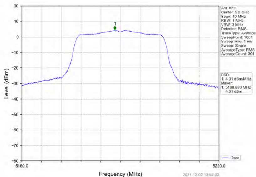
802.11ac(VHT20)_MCH_5200MHz_Ant1_NTNV
