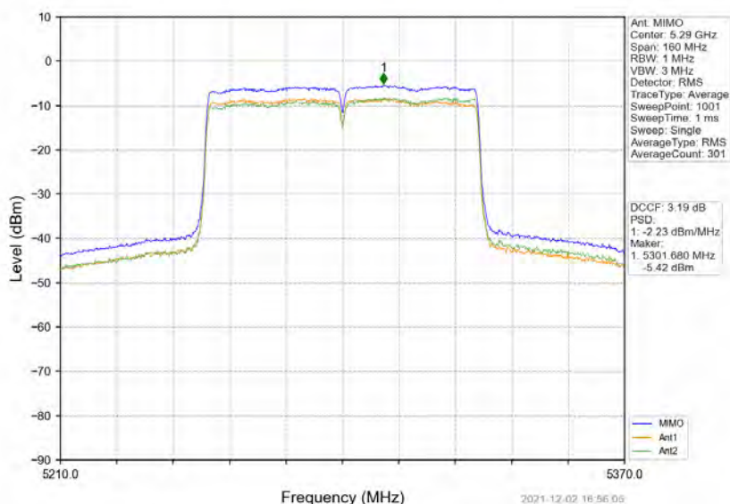
802.11ac(VHT80)_MCH_5290MHz_MIMO_NTNV
