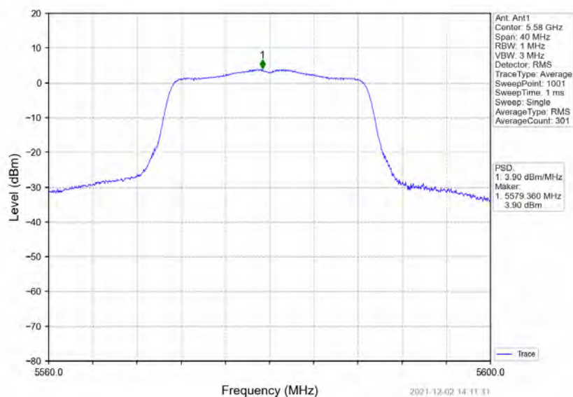
802.11ac(VHT20)_MCH_5580MHz_Ant1_NTNV
