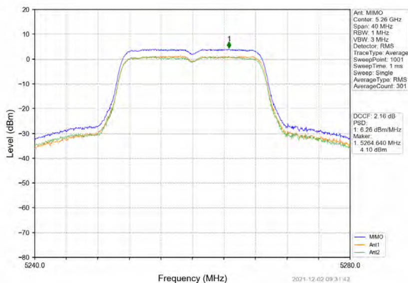
802.11n(HT20)_LCH_5260MHz_MIMO_NTNV
