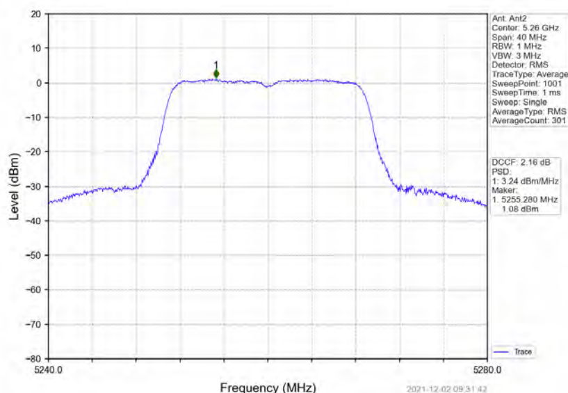
802.11n(HT20)_LCH_5260MHz_MIMO_NTNV
