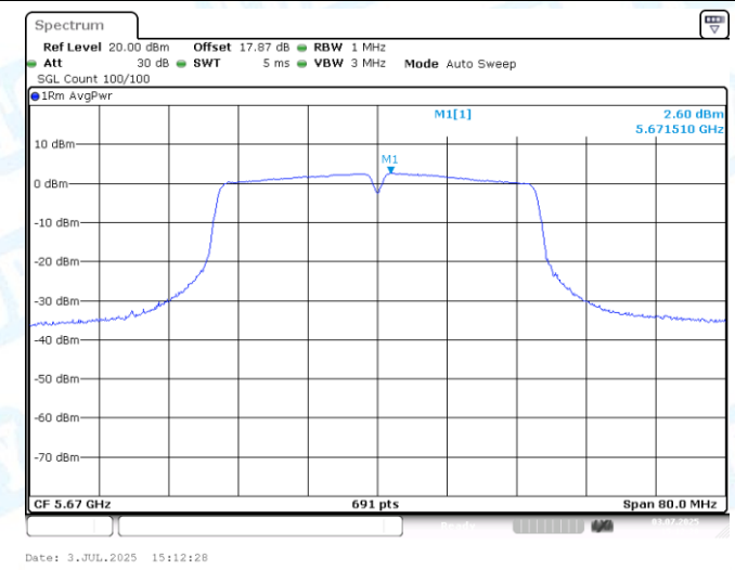
11AC40SISO-Ant1-5670-PASS
