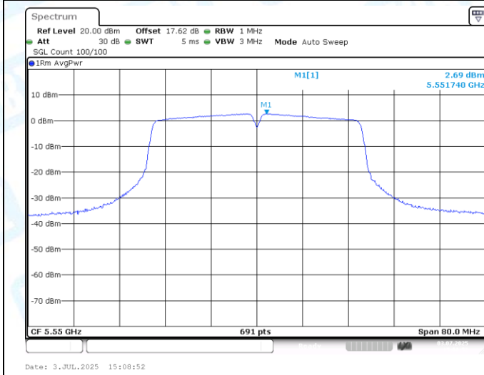
11AC40SISO-Ant1-5550-PASS
