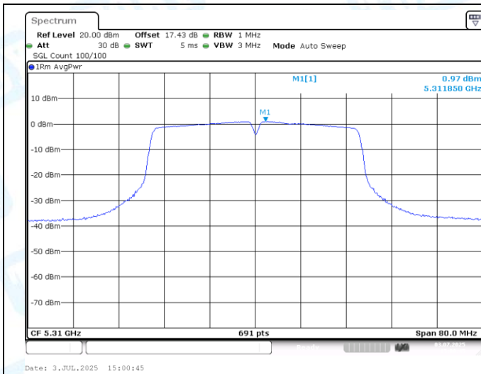
11AC40SISO-Ant1-5310-PASS
