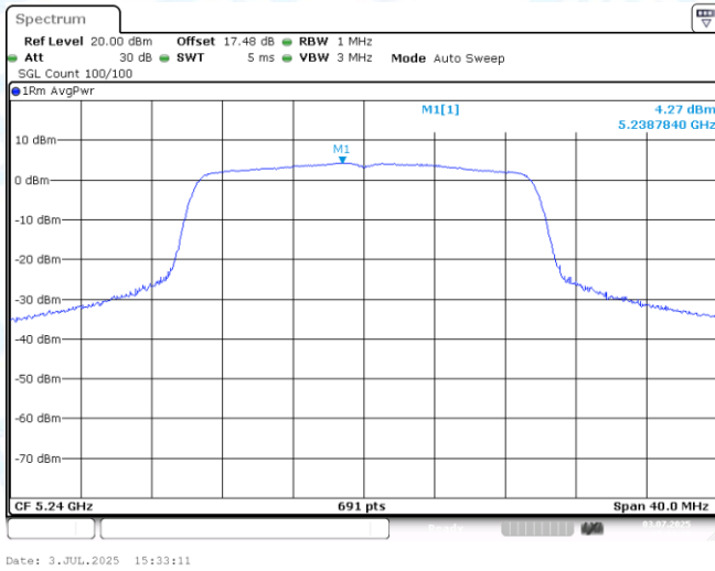
11AX20SISO-Ant1-5240-PASS
