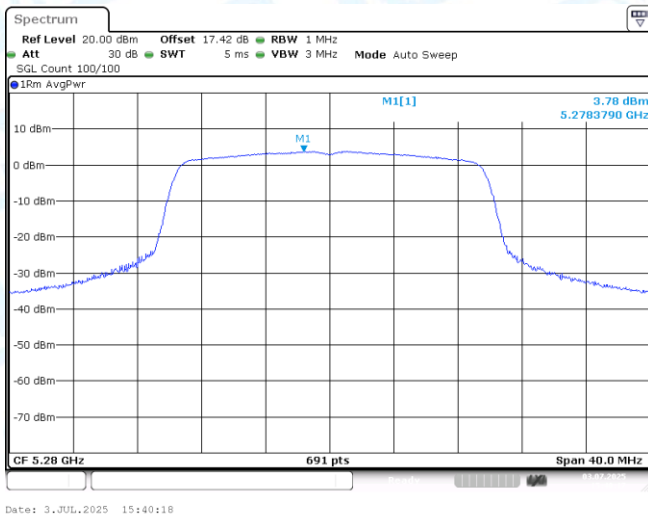
11AX20SISO-Ant1-5280-PASS
