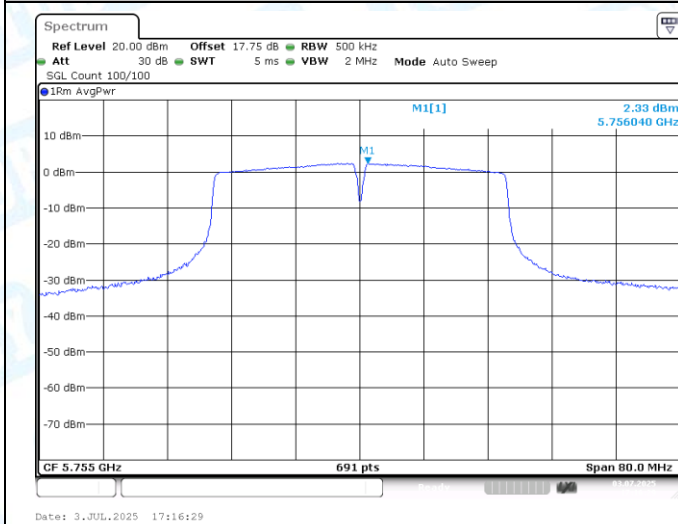
11AC40SISO-Ant1-5755-PASS
