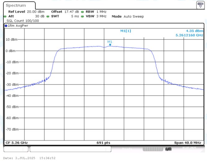
11AX20SISO-Ant1-5260-PASS
