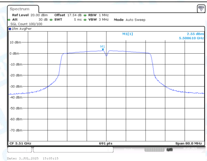
11AC40SISO-Ant1-5510-PASS
