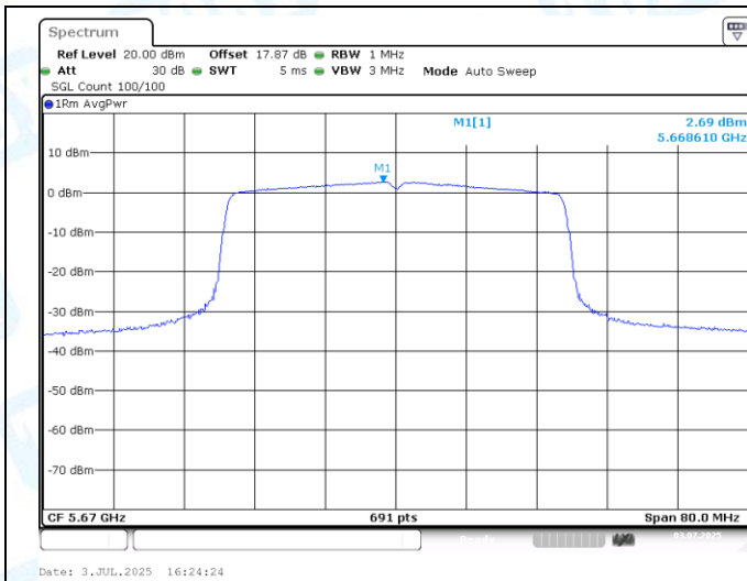
11AX40SISO-Ant1-5670-PASS
