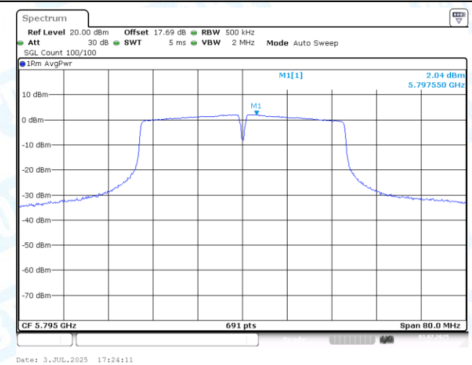
11AC40SISO-Ant1-5795-PASS
