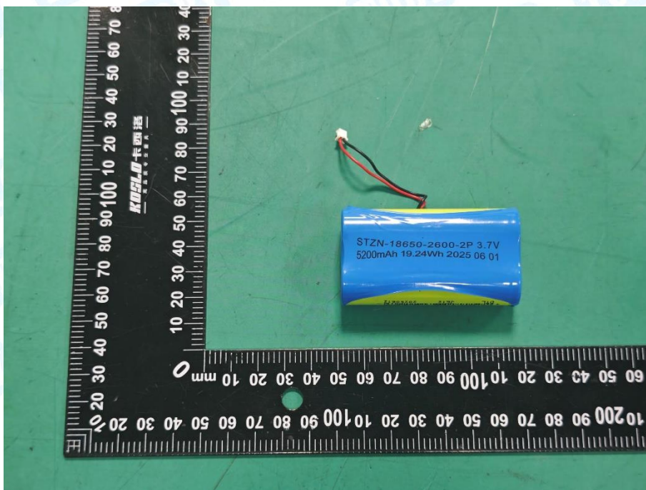
Photo 19 Battery Appearance
