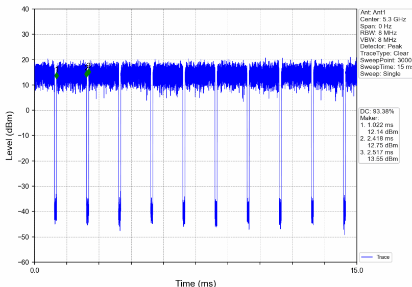
802.11a_HCH_5320MHz_Ant1_NTNV
