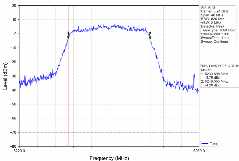
802.11n(HT20)_HCH_5240MHz_Ant2_NTNV
