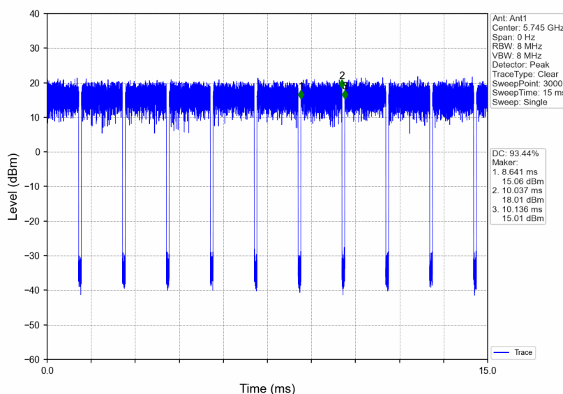
802.11a_LCH_5745MHz_Ant1_NTNV
