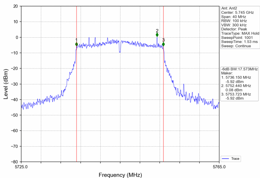
802.11ac(VHT20) LCH_5745MHz_Ant2_NTNV
