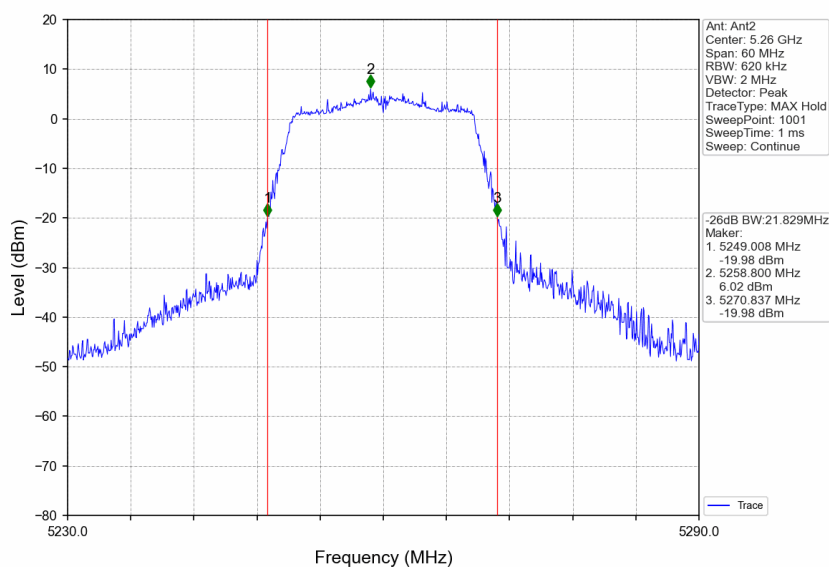
802.11ac(VHT20) LCH_5260MHz_Ant2_NTNV
