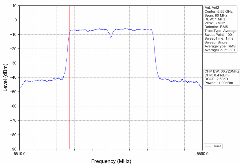
802.11n(HT40)_MCH_5550MHz_Ant2_NTNV
