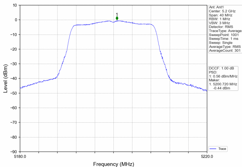
802.11ac(VHT20)_MCH_5200MHz_Ant1_NTNV
