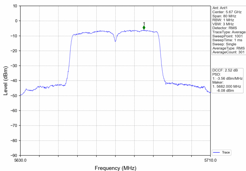
802.11n(HT40)_HCH_5670MHz_Ant1_NTNV
