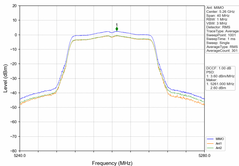
802.11ac(VHT20)_LCH_5260MHz_MIMO_NTNV
