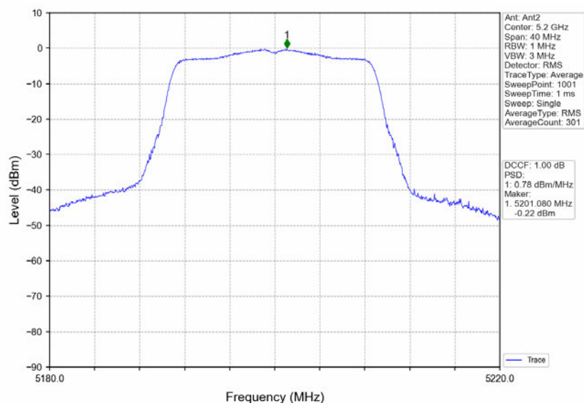
802.11ac(VHT20)_MCH_5200MHz_MIMO_NTNV
