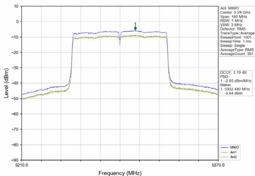
802.11ac(VHT80)_MCH_5290MHz_MIMO_NTNV
