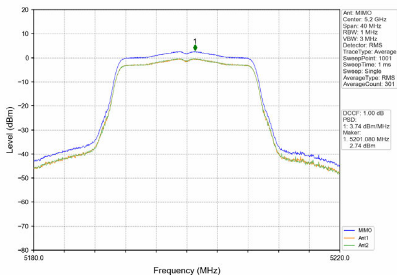
802.11ac(VHT20)_MCH_5200MHz_MIMO_NTNV
