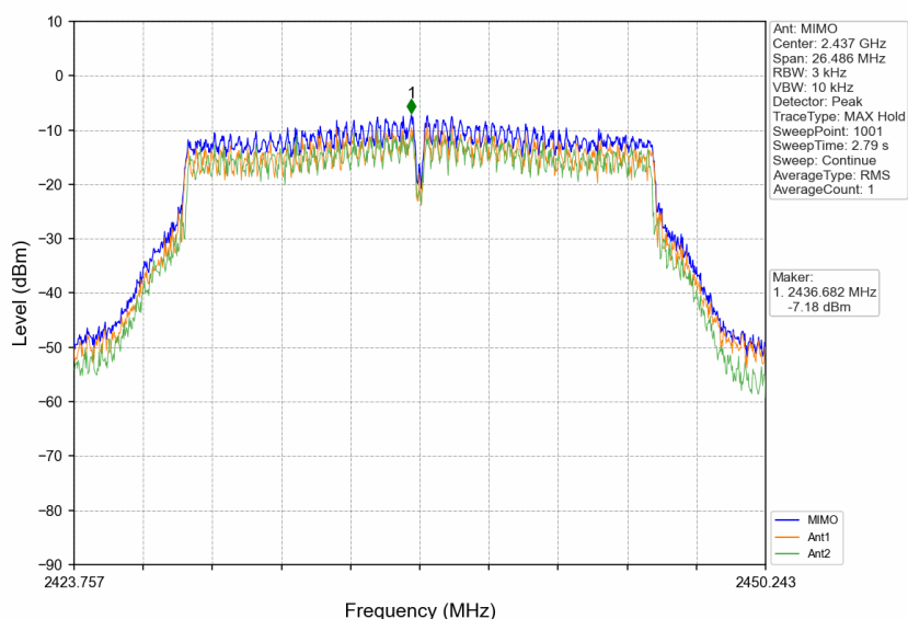
802.11n(HT20)_MCH_2437MHz_MIMO NTN
