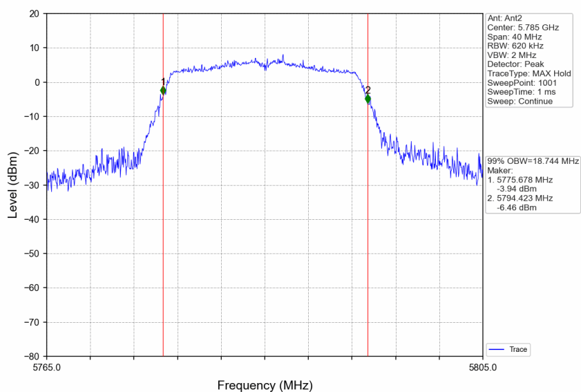
802.11n(HT20)_MCH_5785MHz_Ant2_NTNV
