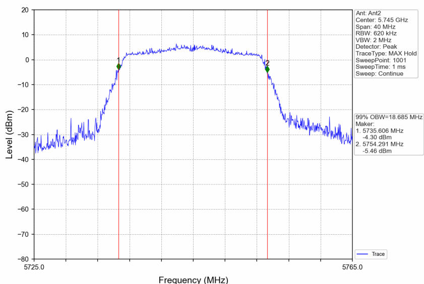
802.11ac(VHT20) LCH_5745MHz_Ant2_NTNV
