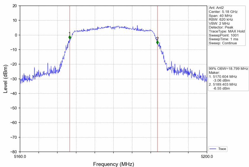
802.11ac(VHT20) LCH_5180MHz_Ant2_NTNV
