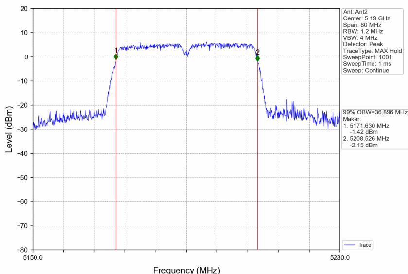
802.11ac(VHT40) LCH_5190MHz_Ant2_NTNV
