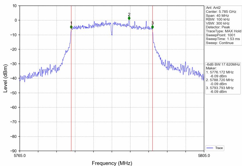
802.11n(HT20)_MCH_5785MHz_Ant2_NTNV
