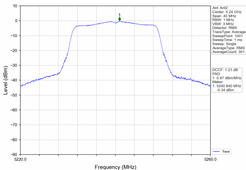
802.11n(HT20)_HCH_5240MHz_Ant2_NTNV
