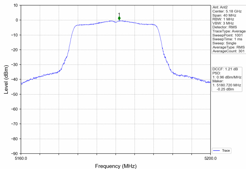
802.11ac(VHT20) LCH_5180MHz_Ant2_NTNV
