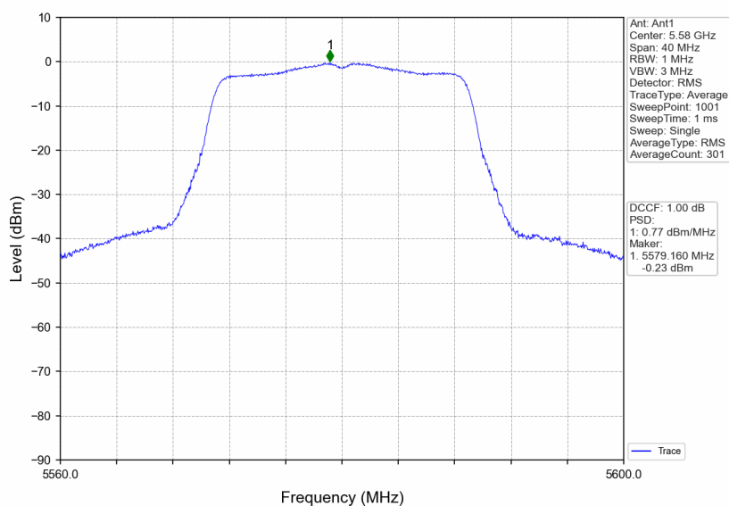
802.11ac(VHT20)_MCH_5580MHz_Ant1_NTNV
