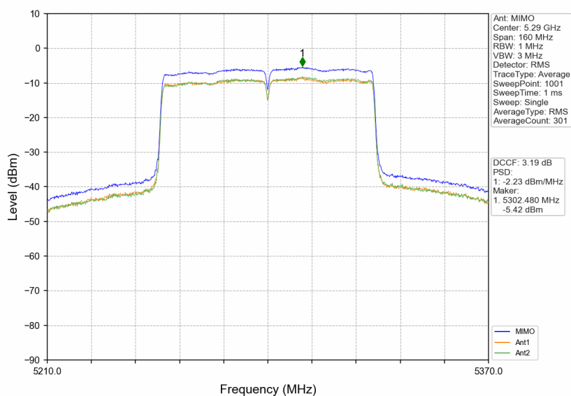
802.11ac(VHT80)_MCH_5290MHz_MIMO_NTNV
