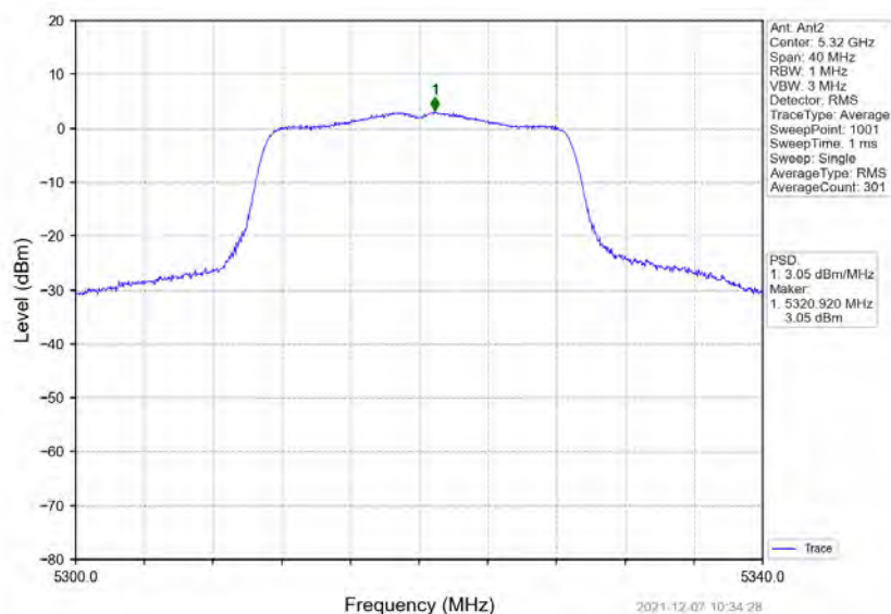
802.11ac(VHT20)_HCH_5320MHz_MIMO_NTNV
