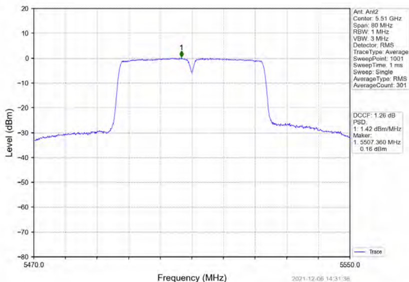
802.11n(HT40)_LCH_5510MHz_MIMO_NTNV
