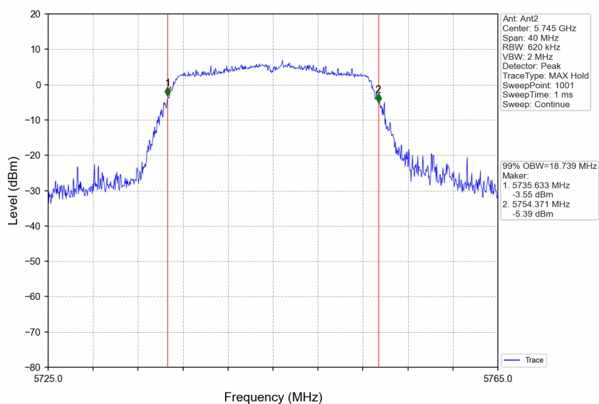
802.11ac(VHT20) LCH_5745MHz_Ant2_NTNV
