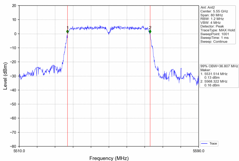
802.11n(HT40)_MCH_5550MHz_Ant2_NTNV
