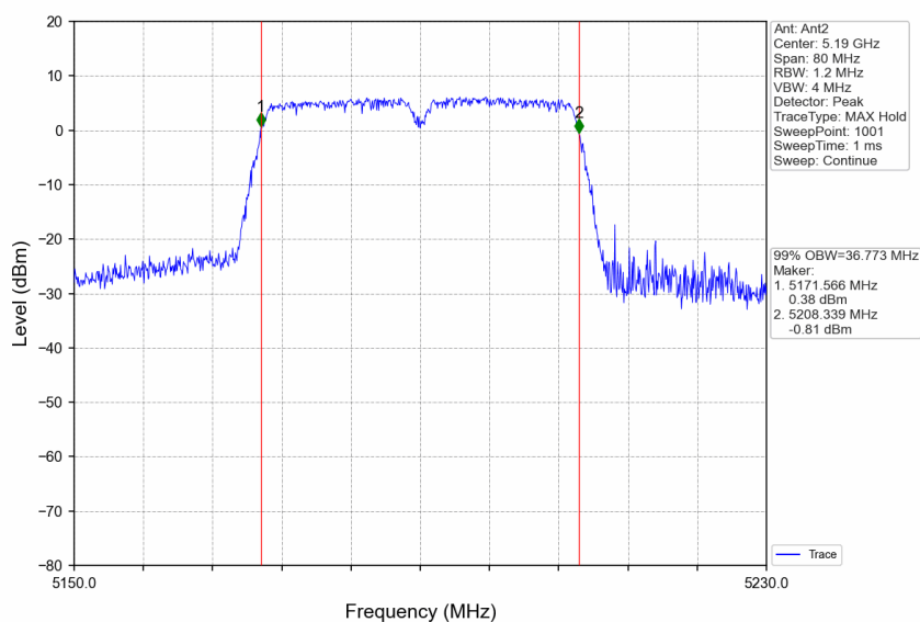
802.11ac(VHT40) LCH_5190MHz_Ant2_NTNV
