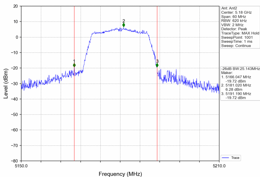
802.11ac(VHT20) LCH_5180MHz_Ant2_NTNV
