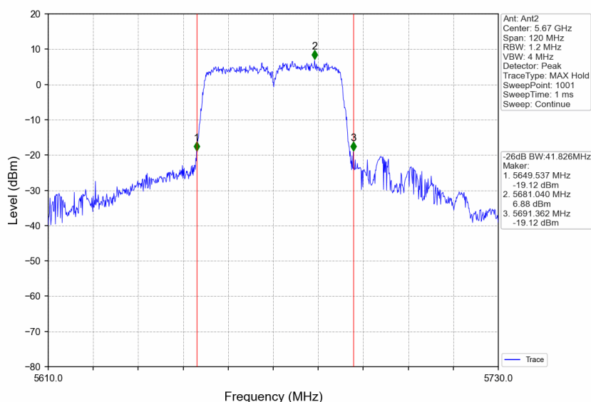
802.11n(HT40)_HCH_5670MHz_Ant2_NTNV
