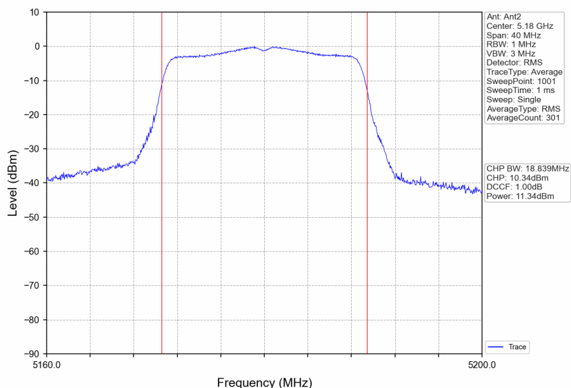
802.11ac(VHT20) LCH_5180MHz_Ant2_NTNV
