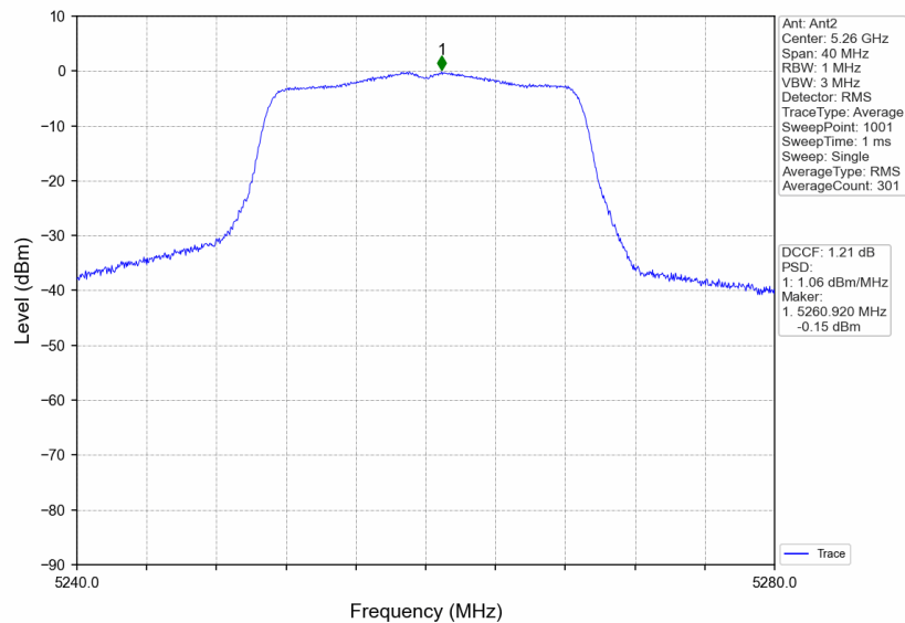
802.11ac(VHT20)_LCH_5260MHz_MIMO_NTNV
