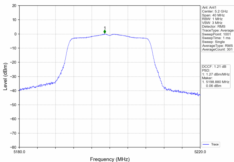
802.11ac(VHT20)_MCH_5200MHz_Ant1_NTNV
