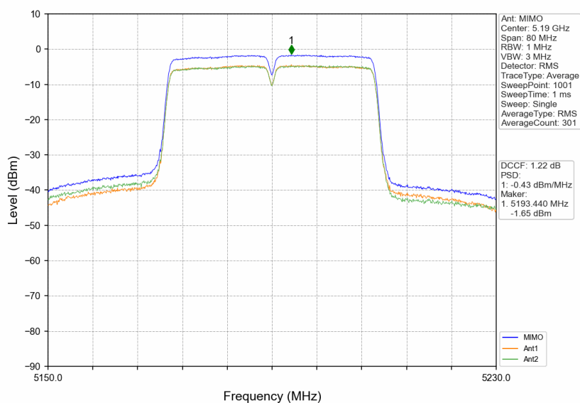
802.11ac(VHT40)_LCH_5190MHz_MIMO_NTNV
