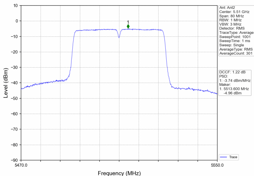
802.11ac(VHT40)_LCH_5510MHz_MIMO_NTNV
