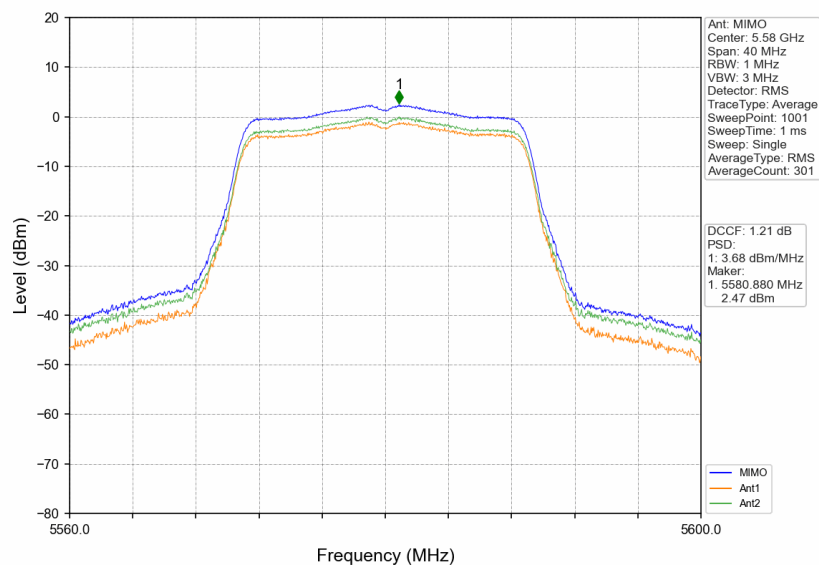
802.11ac(VHT20)_MCH_5580MHz_MIMO_NTNV
