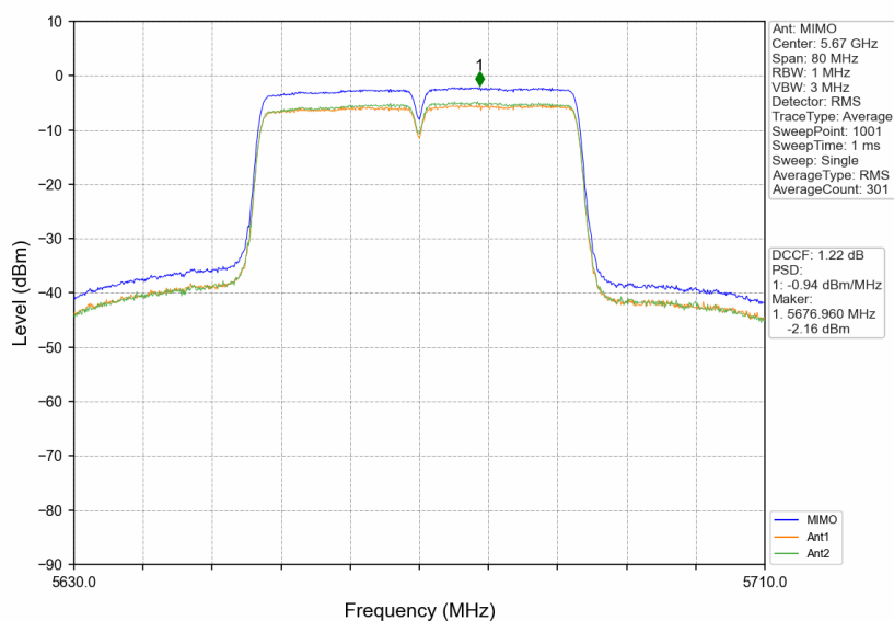
802.11ac(VHT40) HCH_5670MHz_MIMO_NTNV
