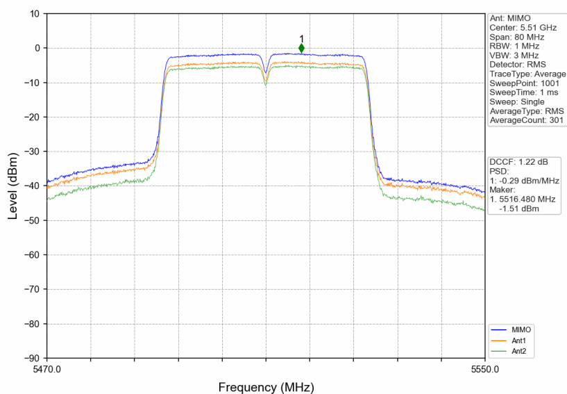
802.11ac(VHT40)_LCH_5510MHz_MIMO_NTNV
