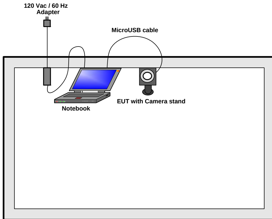
Test Setup Diagram - Radiated Emission Above 1GHz (Mode 1)
