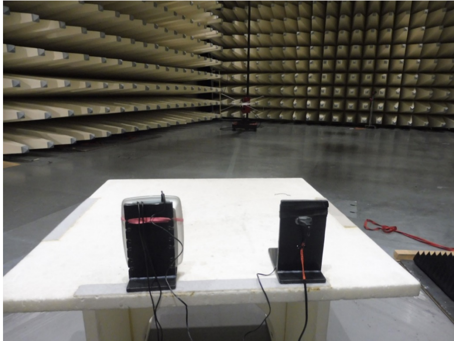
Photo 1: Radiated Emission
