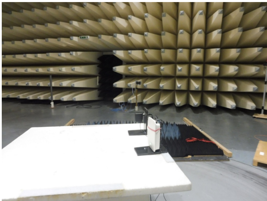
Photo 2: Radiated Emission
