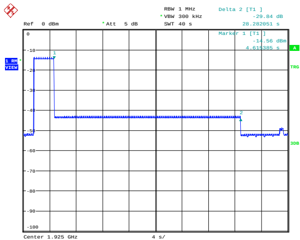
Activating EUT, acknowledgement blocked from companion
