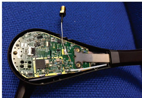
Figure 7: Headset test configuration - test cable connection to PCB
