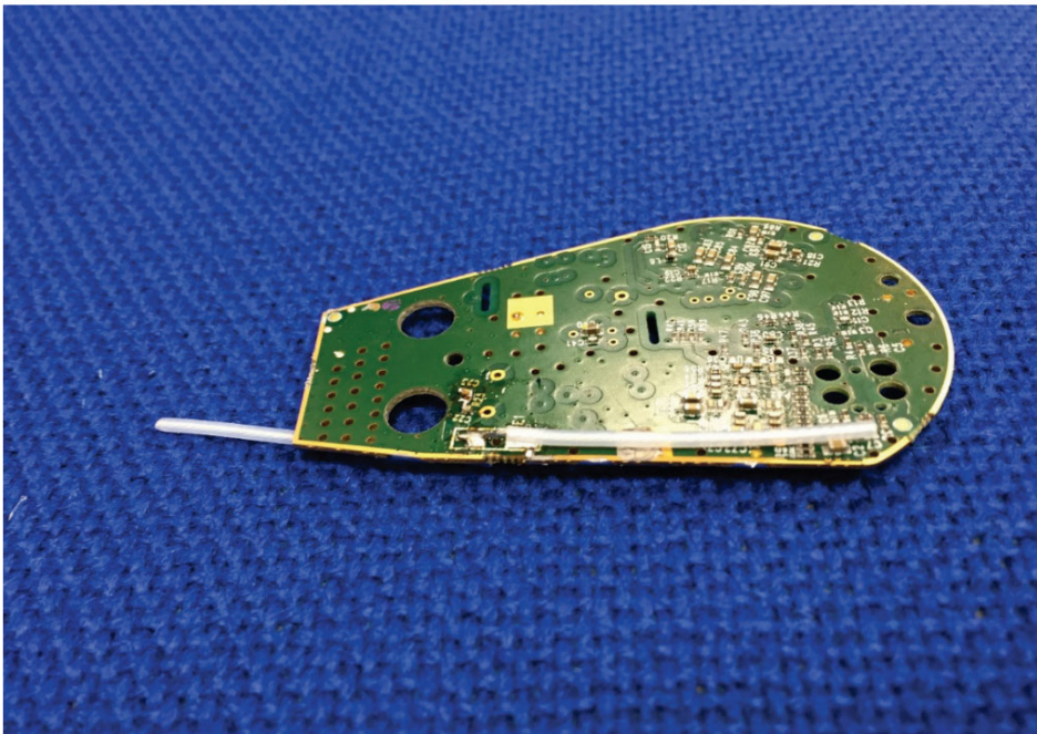
Figure 11: Headset test configuration – Bottom of PCB - side view
