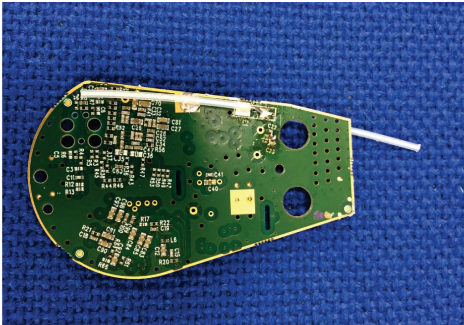
Figure 10: Headset test configuration – Bottom of PCB
