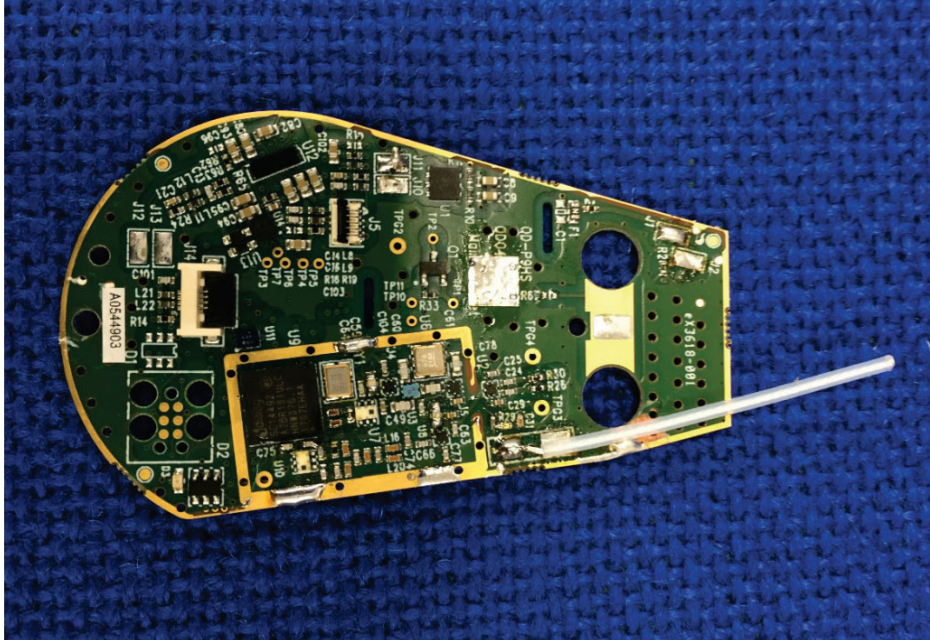
Figure 8: Headset test configuration – Top of PCB
