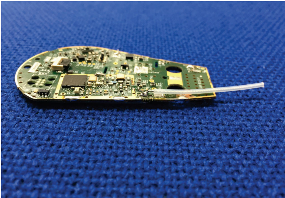
Figure 9: Headset test configuration – Top of PCB - side view
