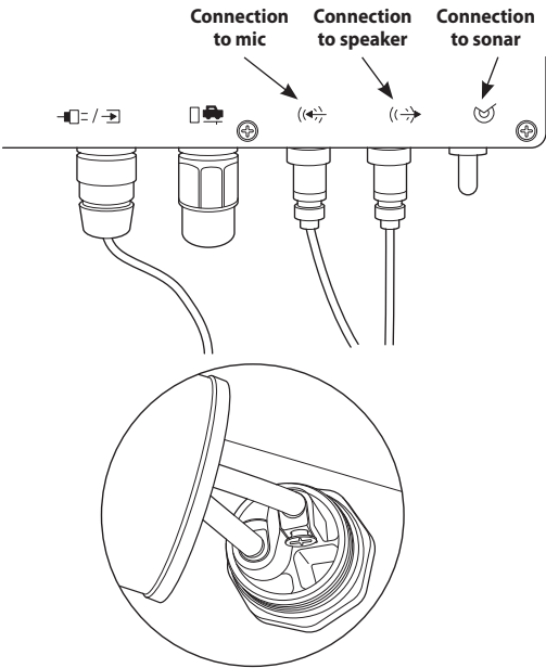
Figure 5 - Loop connection
