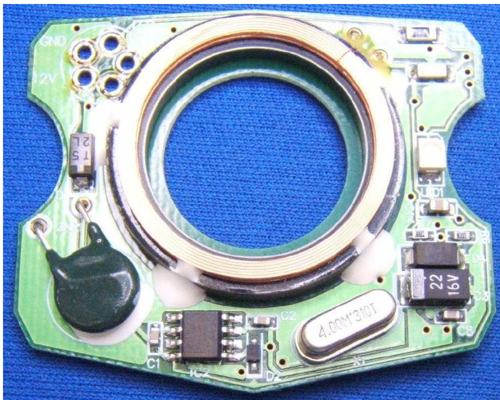
Circuit Board without Cable (Back)
