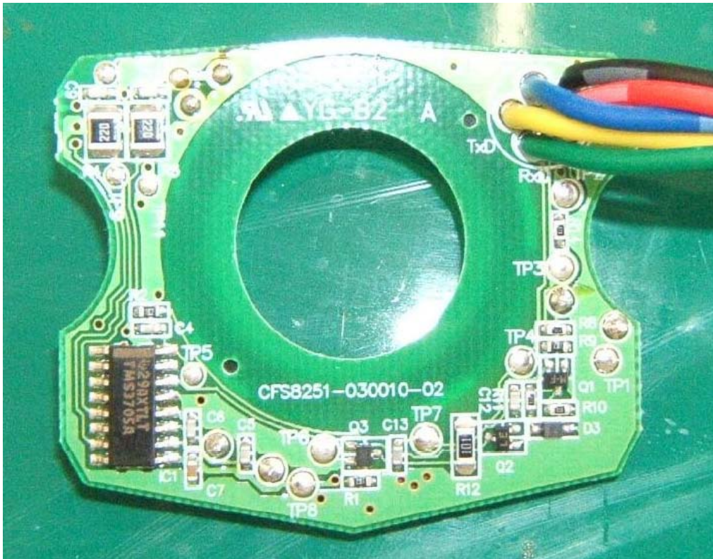
Circuit Board with Cable (Front)
