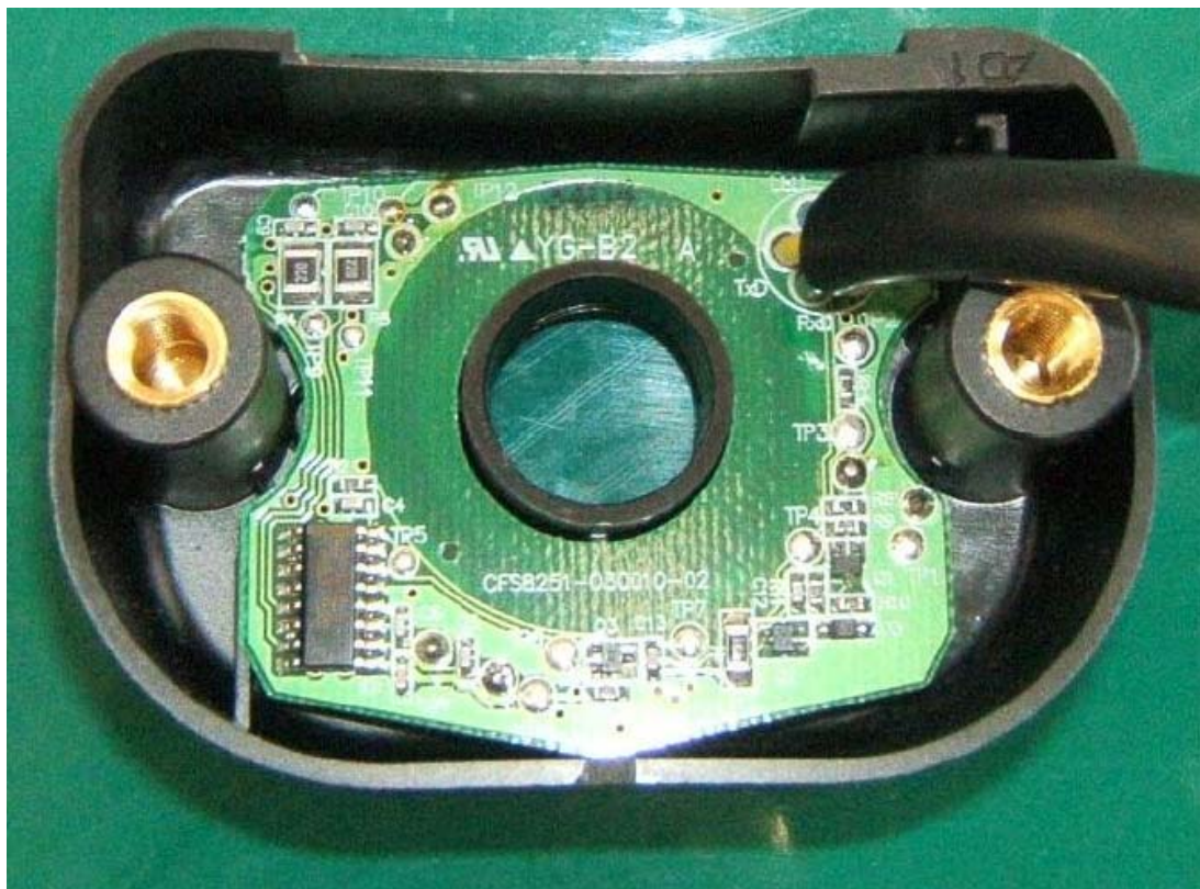
Open View with Circuit Board
