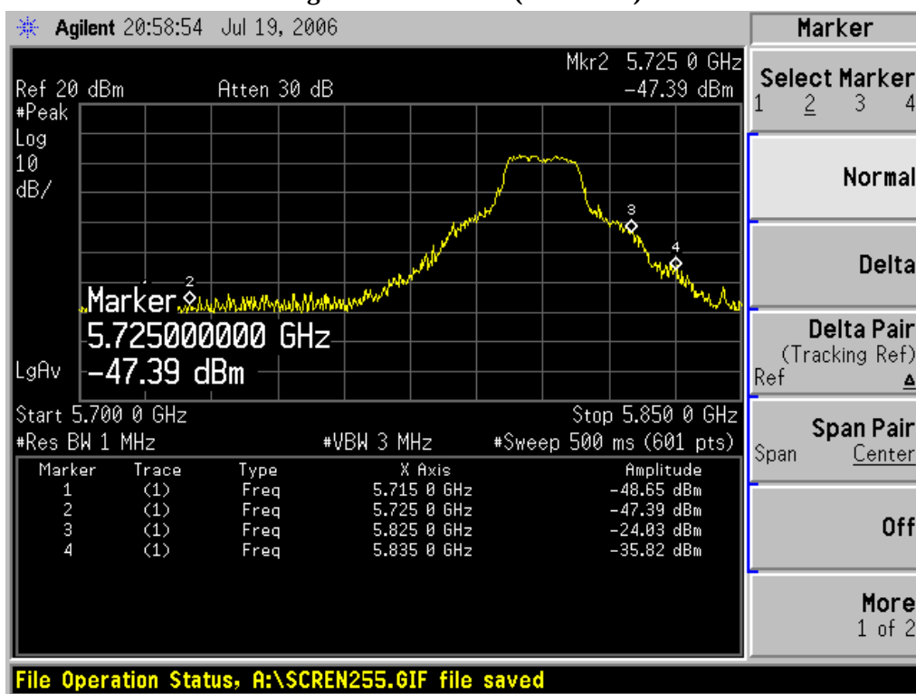
Figure Channel 161 (5805MHz)
