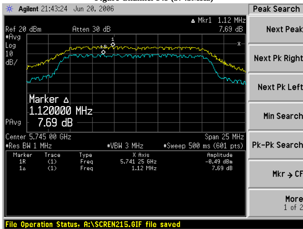
Figure Channel 149 (5745MHz)
