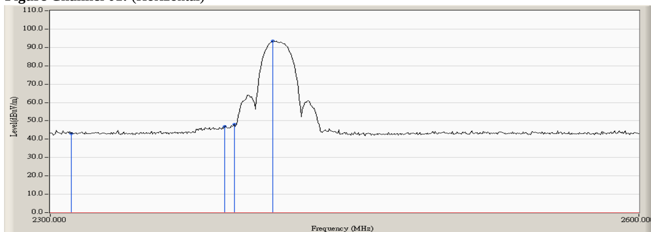
Figure Channel 01: (Horizontal)
