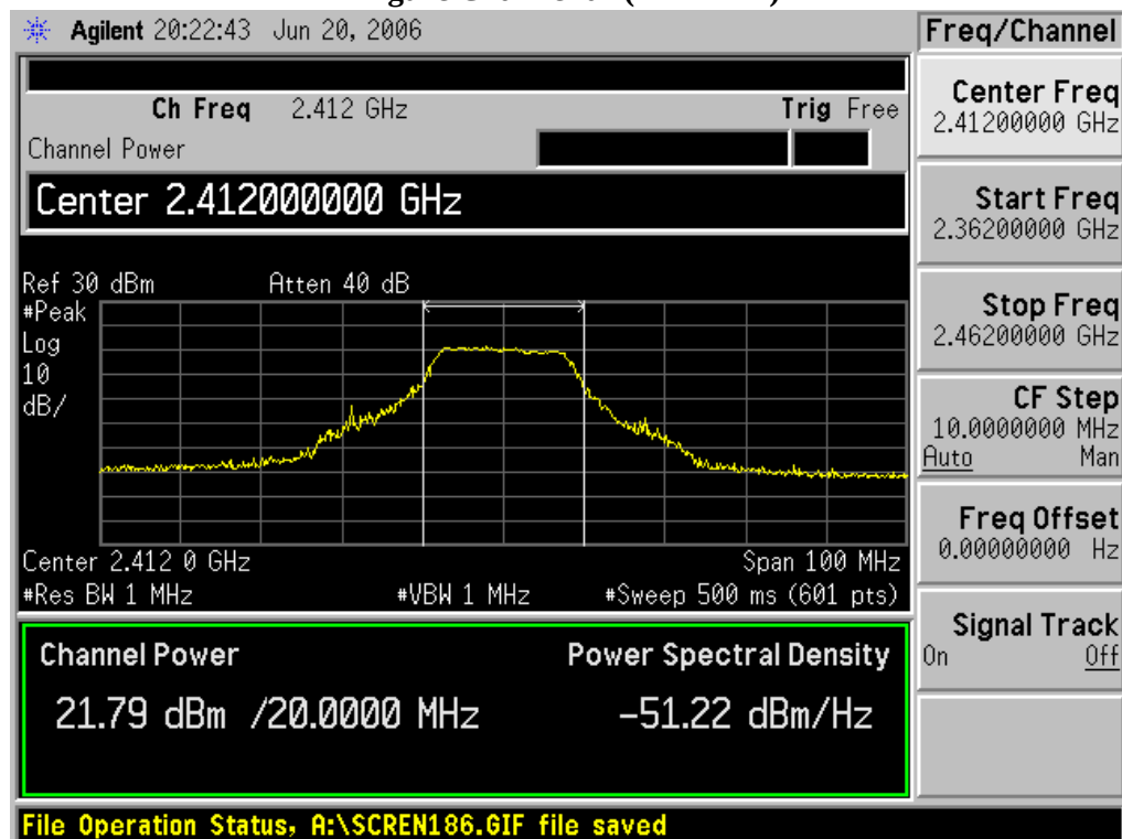
Figure Channel 01 (2412MHz)
