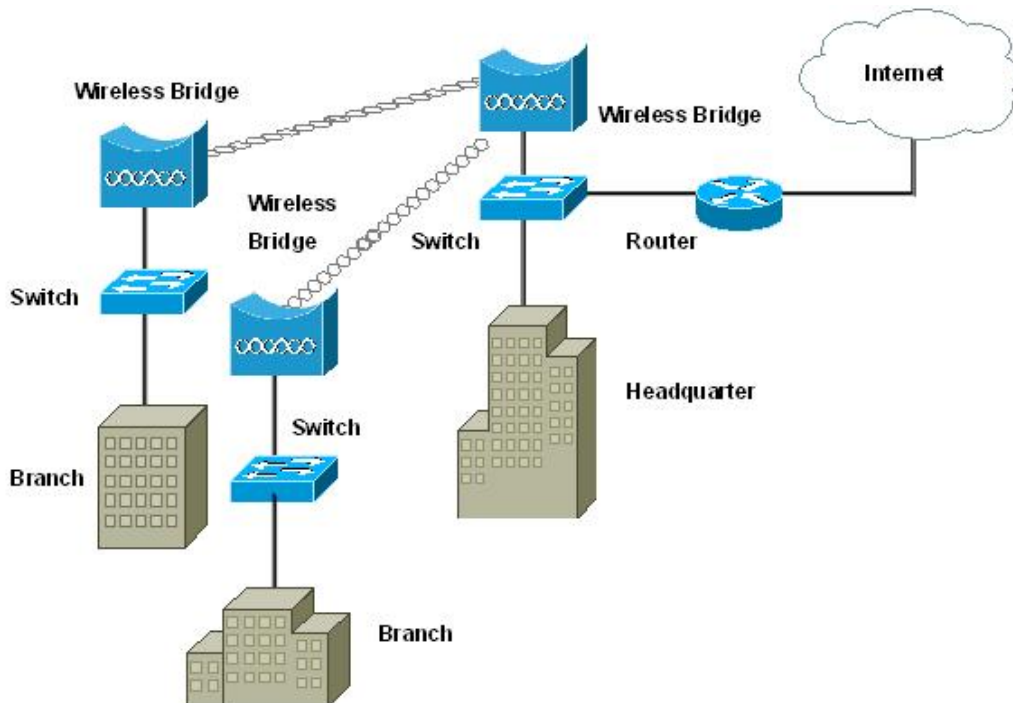
Figure 4 Point to Multi Point
