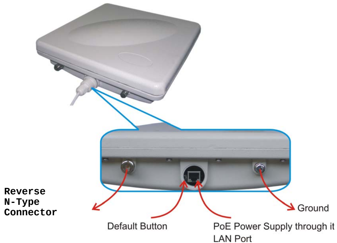
Figure 2 ZA-5000-E
