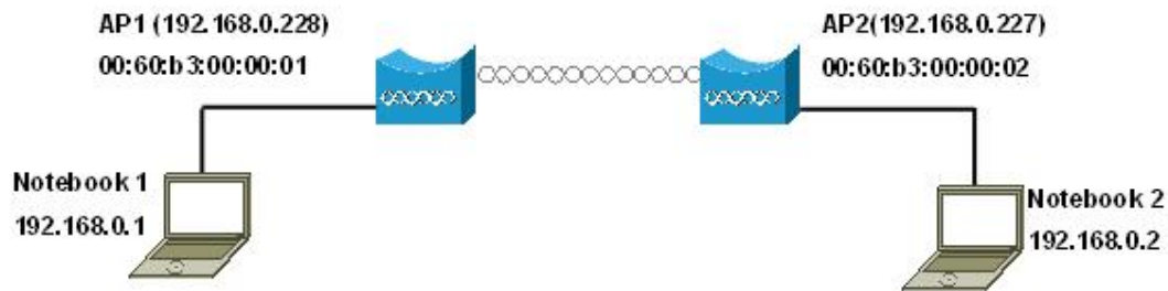
Figure 12 Point to Point Connection
