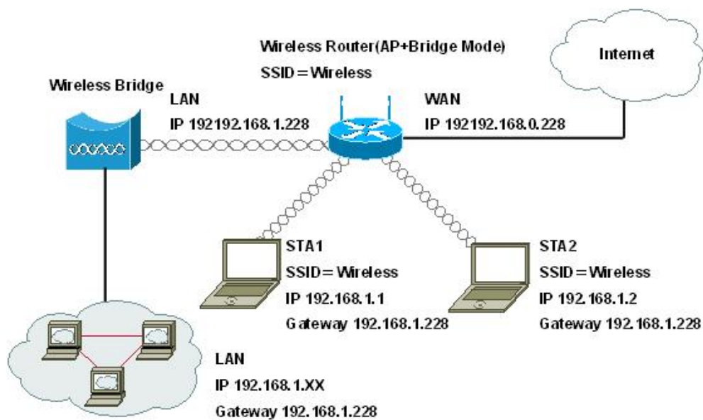
Figure 26 “AP + Bridge” Router
