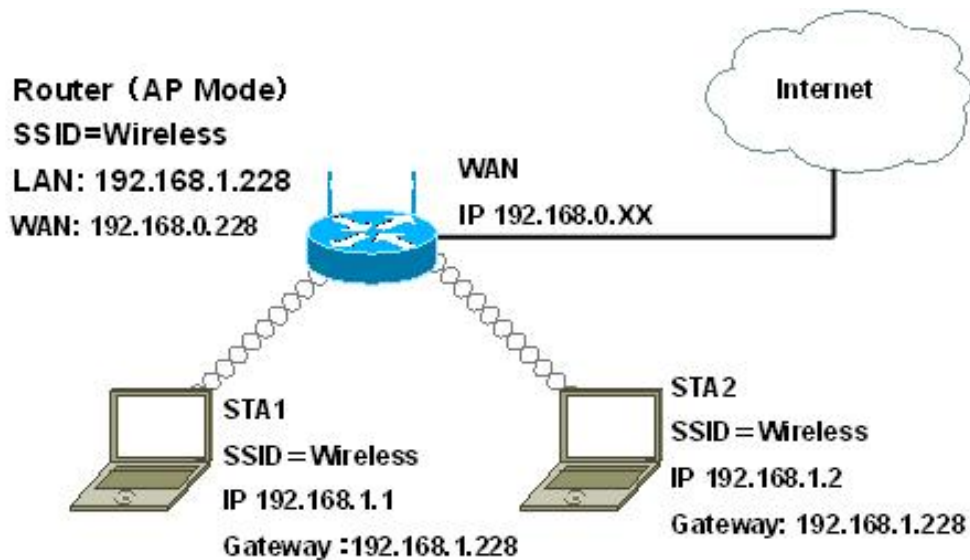
Figure 25 AP Router
