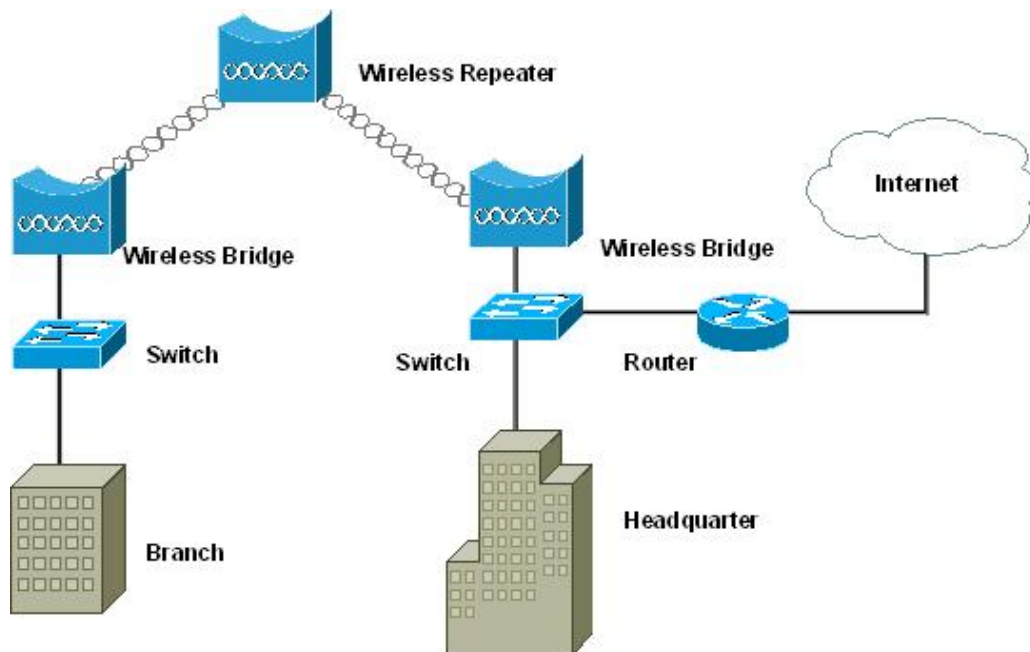
Figure 5 Wireless Repeater
