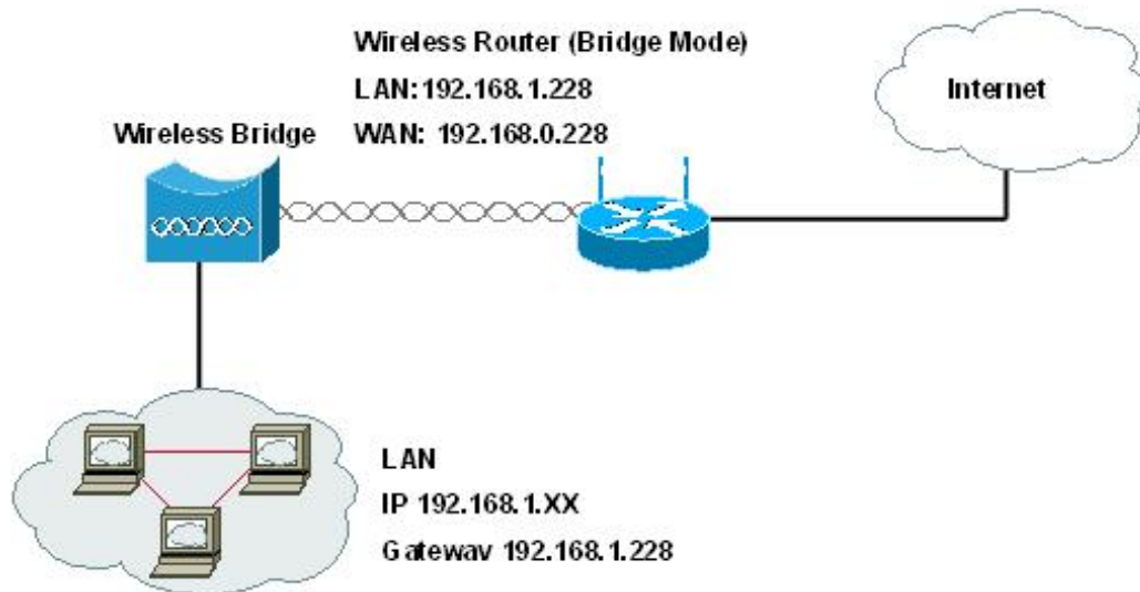
Figure 23 Wireless Router (Bridge Mode)—WAN on Ethernet
