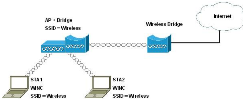
Figure 32 “AP + Bridge” Mode Application
