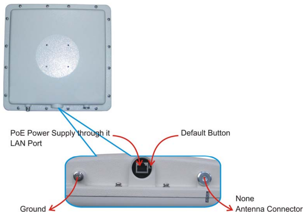
Figure 1 ZA-5000-I
