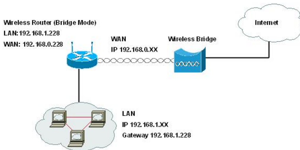
Figure 24 Wireless Router (Bridge Mode)—WAN on Wireless
